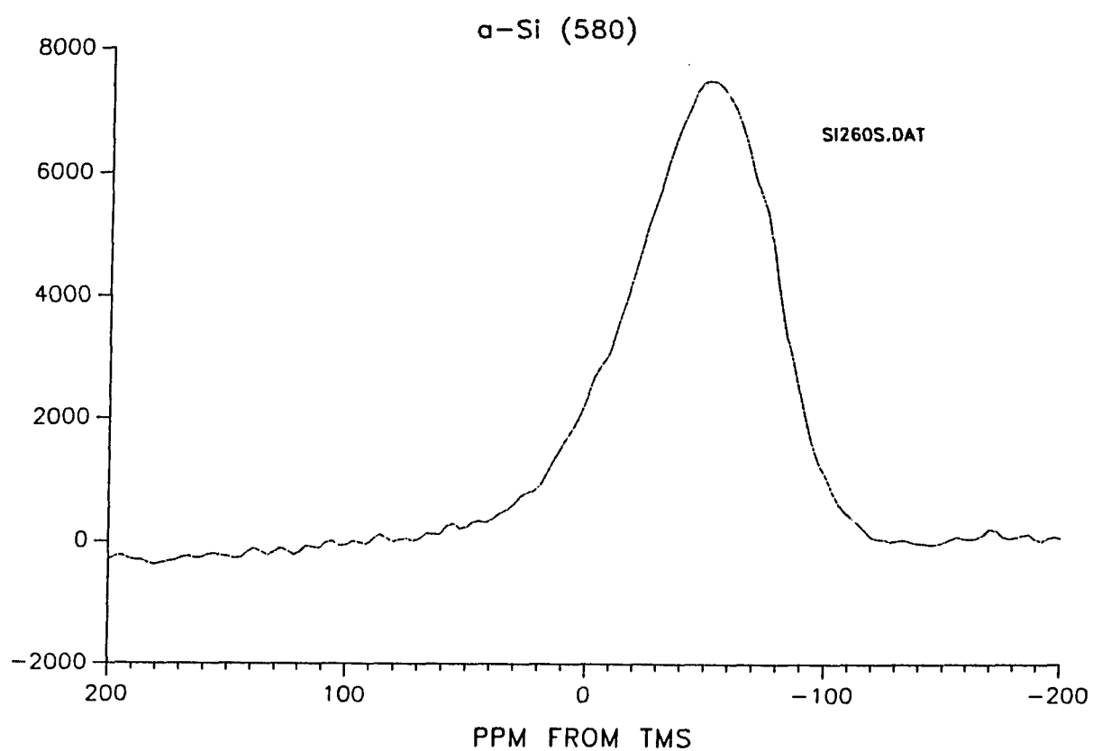
Figure 7. MAS NMR spectrum of a-Si after annealing at 580 °C
