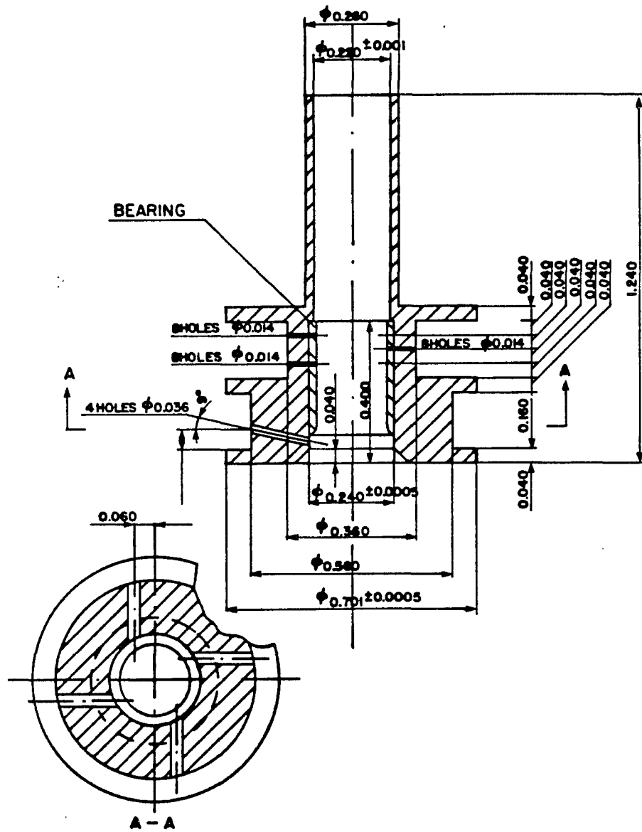
Figure 3. Stator and air bearing ring
