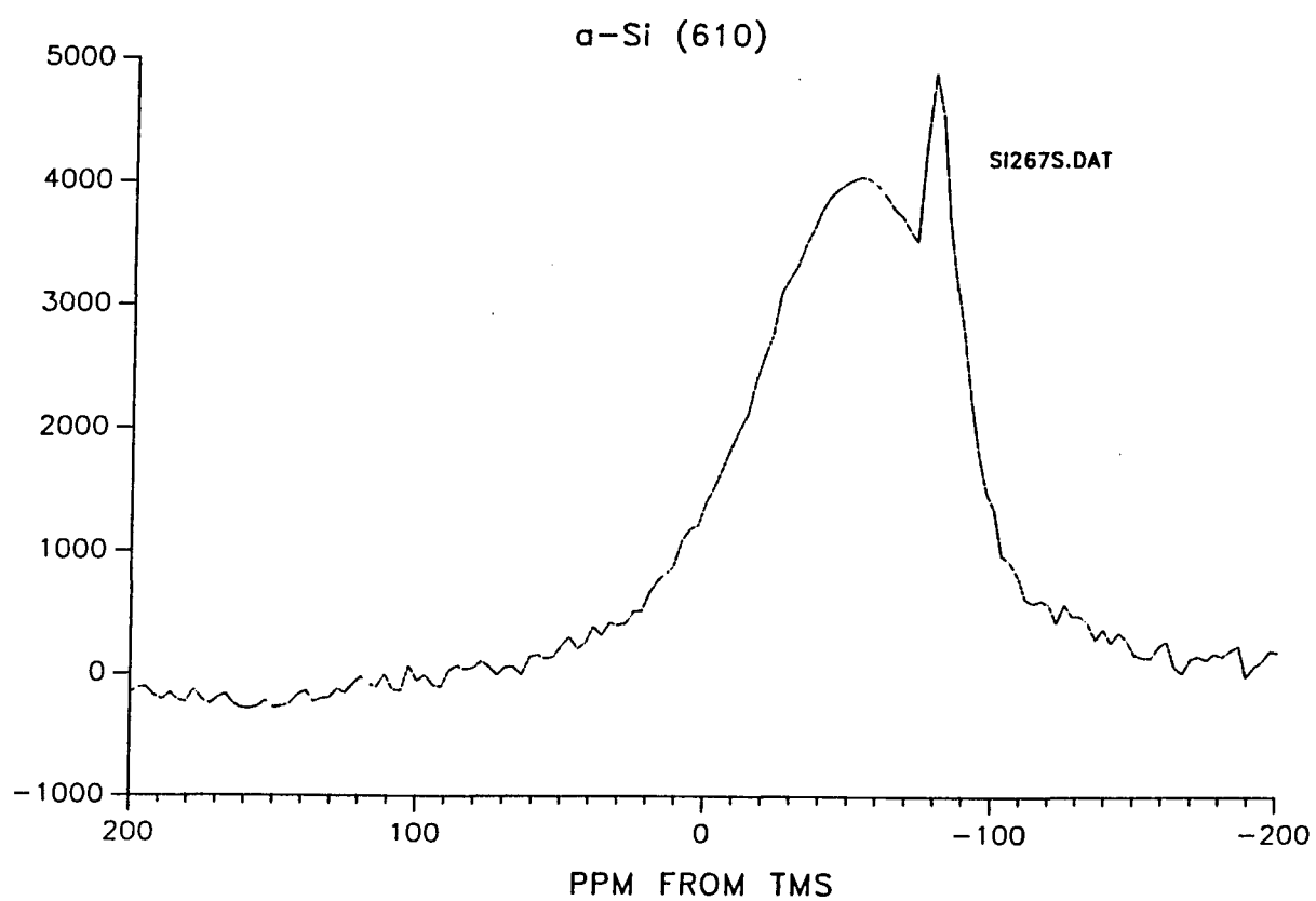
Figure 8. MAS NMR spectrum of a-Si after annealing at 610 °C
