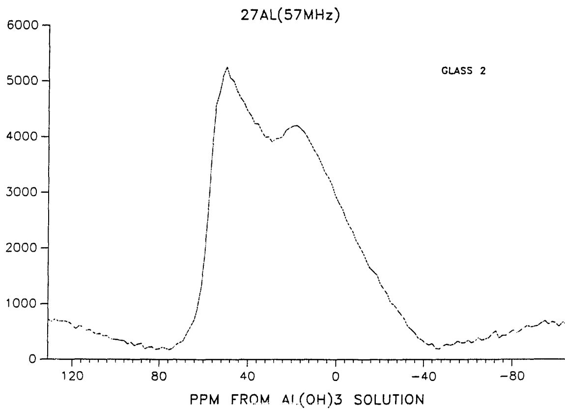
Figure 15. ^{27}\text{Al} MAS NMR spectrum of glass 2 taken at 57 MHz
