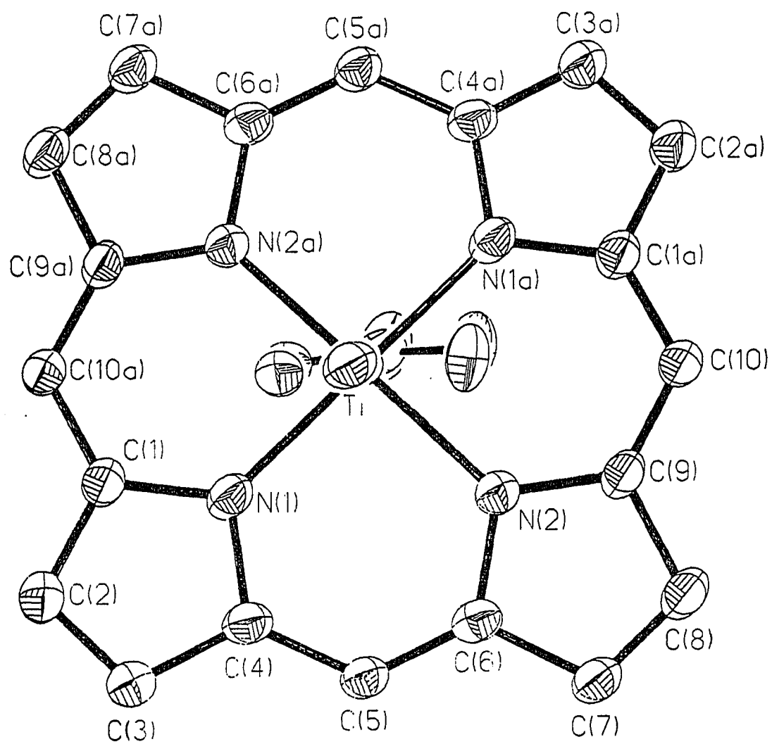
Figure 2. Axial view of (\text{TTP})\text{Ti}(\text{NC}_3\text{H}_4\text{-}p\text{-CH}_3)_2 showing relationship of the picoline ring to the porphyrin plane
