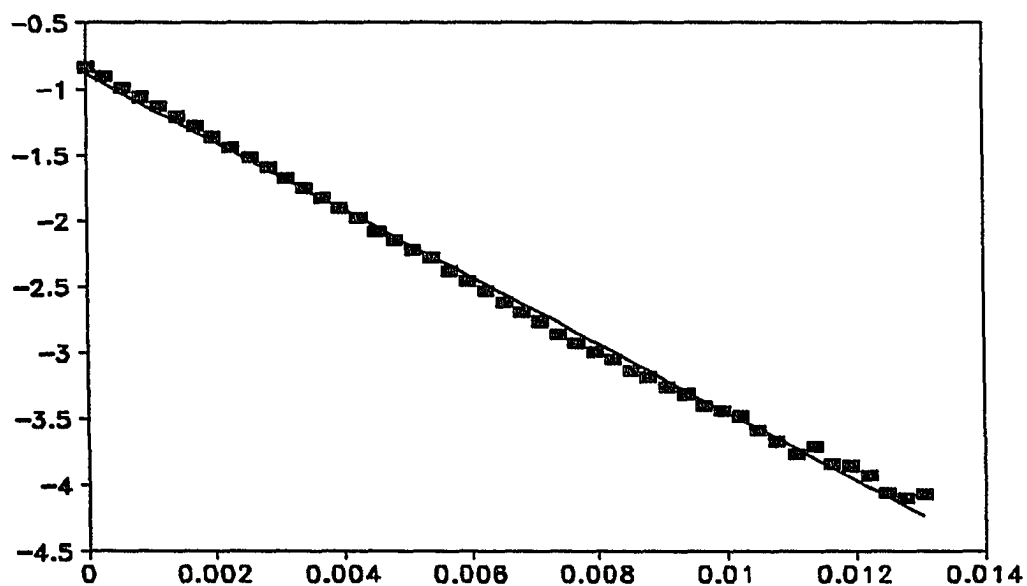
Figure 2. Plot of \ln[\Delta/(\alpha + \Delta(1 - 1/K))] vs. \alpha t for figure 1, k_t = 256 \pm 2 \text{ M}^{-1}\text{s}^{-1}
