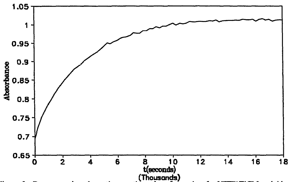
Figure 3. Representative absorption vs. time plot of equation 6. [(\text{TTP})\text{TiCl}_2] = 4.44 \times 10^{-5} M, [(\text{OEP})\text{Ti=O}] = 4.41 \times 10^{-5} M, in \text{CHCl}_3 at 20^\circ\text{C}
