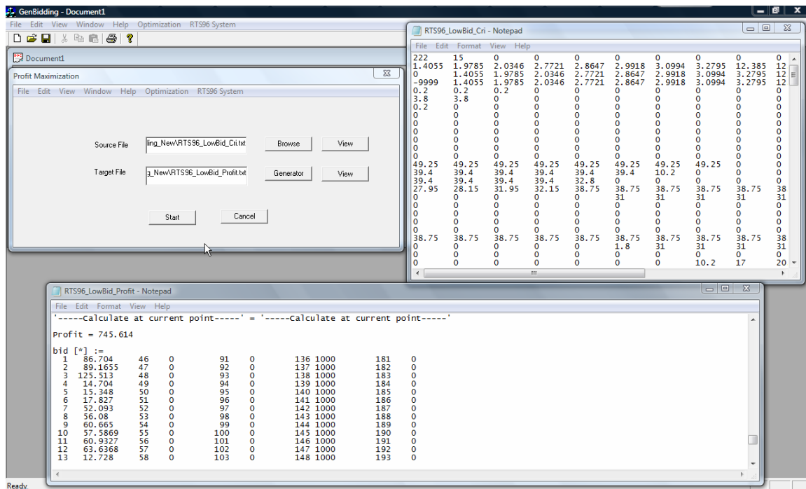
Figure 58: Profit Maximization
