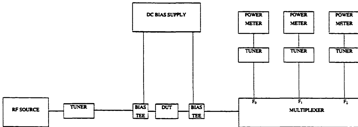
Figure 2-3 Simple harmonic load pull setup
