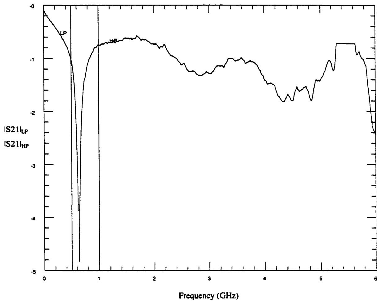
Figure 6-5 Response in the pass bands for the diplexer
