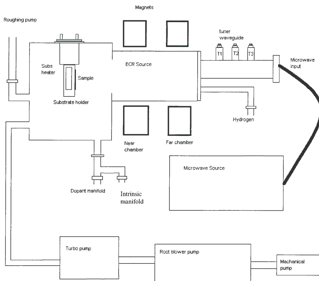
Figure 2.1: ECR system
