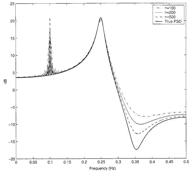
Fig. 4 Average of FT(n) theoretical spectra for the range 1 \rightarrow n_{\max} for n_{\max}=100, 200 and 500
