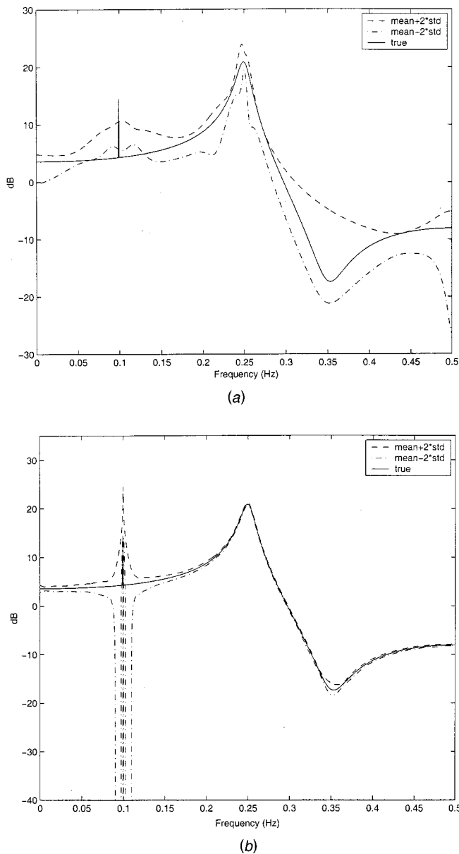
Fig. 2 (a) 2- \sigma curves for an average of 6 AR( n ) spectra, n = 5:1:10 ; (b) 2- \sigma curves for an average of 81 AR( n ) spectra, n = 20:1:100 .
