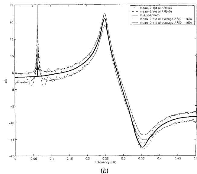
Fig. 8 (a) Evaluation of the variance expression in (28) as a function of model order at a noise frequency. Also shown is the estimated variability of the average of AR spectra (See Section 5 for related discussion). (b) Comparison of predicted (using (28)) 2- \sigma regions associated with an AR(40) model, and an average of AR(p) models for p=2:160 . Also shown is the estimated variability of the average of AR spectra (see Section 5 for related discussion).
