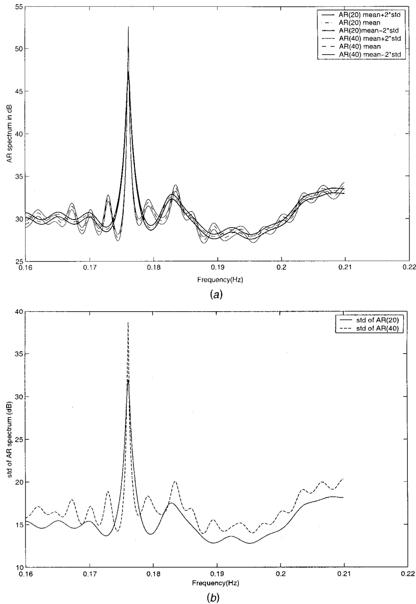
Fig. 12 (a) Comparison of 95% (or 2\sigma ) confidence interval of AR( n ) for n = 20 and 40 for Westland data, (b) Comparison of standard deviation of AR( n ) spectral estimates for n = 20 and 40 for Westland data.
