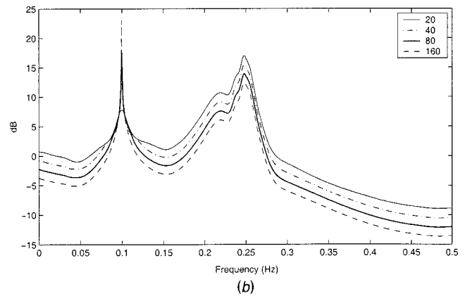
Fig. 6 Arithmetic (a) mean and (b) standard deviation of collection of \{\text{AR}(k): k=2, m\} spectra for m=20, 40, 80 , and 160
