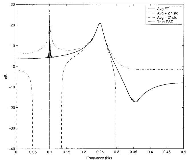
Fig. 1 Arithmetic mean and 2- \sigma curves corresponding to use of a family of theoretical FT( n ) spectra. [Note: Where not shown, the lower 2- \sigma curve is -\infty .]
