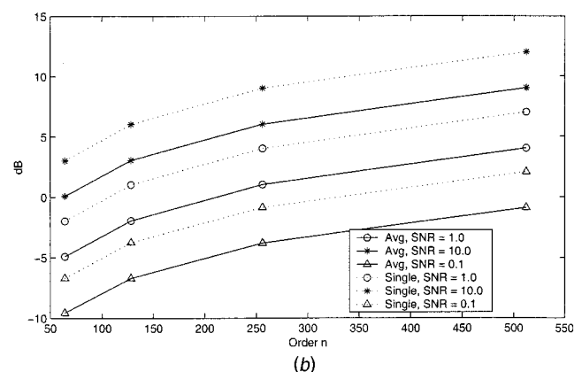
Fig. 9 (a) Comparison of statistical standard deviation of single order PER( n ) and the averaged PER( n ) spectral estimates for selected order n at nontone frequency f=0.1 Hz. (b) Comparison of statistical standard deviation of single order PER( n ) and the averaged PER( n ) spectral estimates for selected order n at tone frequency f=0.3 Hz.
