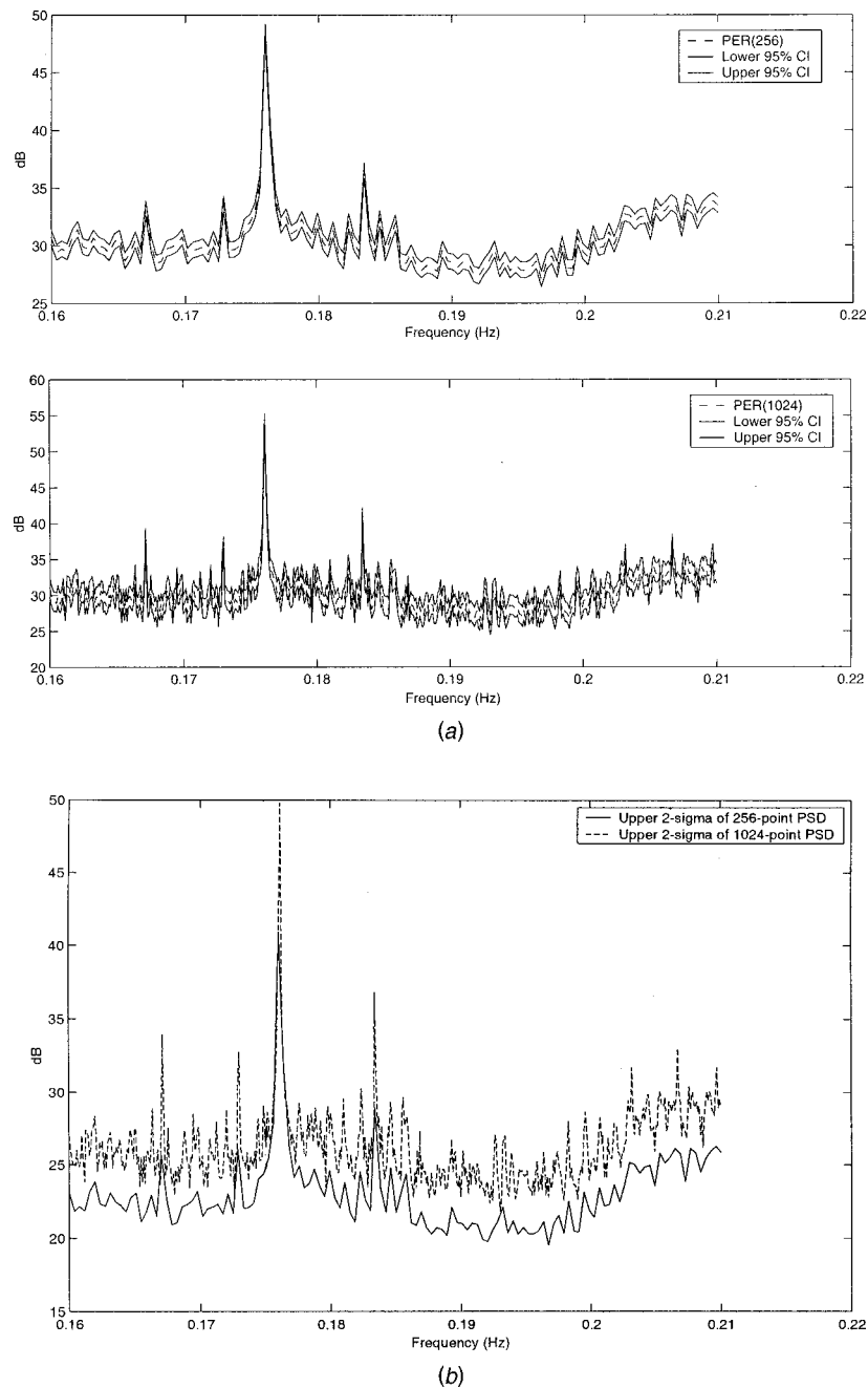
Fig. 11 (a) Comparison of 95% (or 2\sigma ) confidence interval of PER( n ) for n = 256 and 1024 for Westland data. (b) Comparison of 2-sigma of PER( n ) for n = 256 and 1024 for Westland data.
