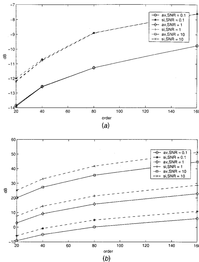
Fig. 10 (a) Comparison of statistical standard deviation of single order \overline{\text{AR}}(n) and the averaged \overline{\text{AR}}(n) spectral estimates for selected order n at non-tone frequency f=0.1 Hz. (b) Comparison of statistical standard deviation of single order \overline{\text{AR}}(n) and the averaged \overline{\text{AR}}(n) spectral estimates for selected order n at tone frequency f=0.3 Hz.
