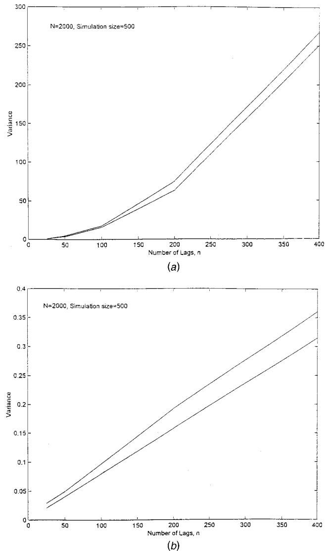
Fig. 7 (a) Comparison of simulation results against predictions (25) at tone's frequency f=0.25 Hz, (b) Comparison of simulation results against predictions (25) at noise frequency f=0.1 Hz.
