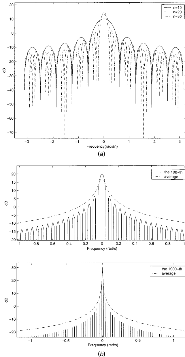
Fig. 5 (a) Example of Fejer kernel for n=10, 20 and 30 in dB; (b) comparison of the n th and the average of the first n Fejer's kernels for n=100 and 1000 .
