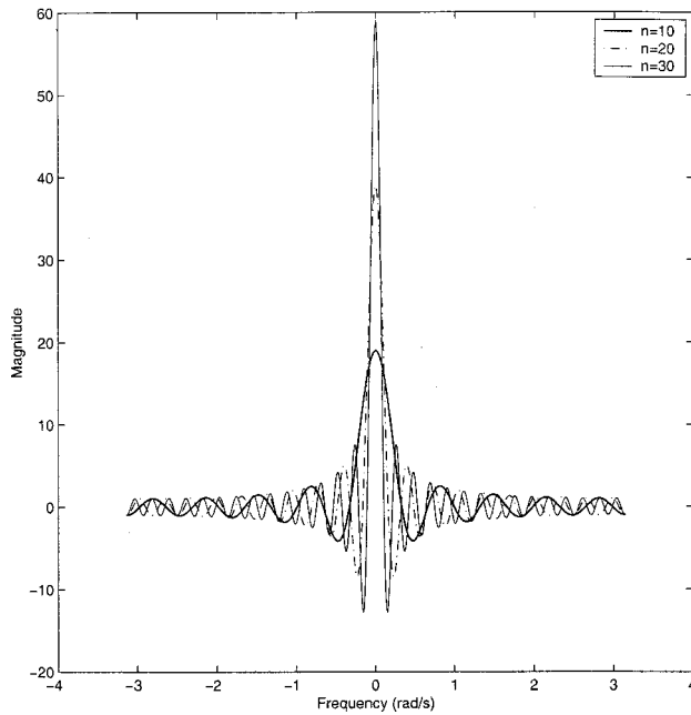
Fig. 3 Example of Dirichlet kernel for n=10, 20 , and 30
