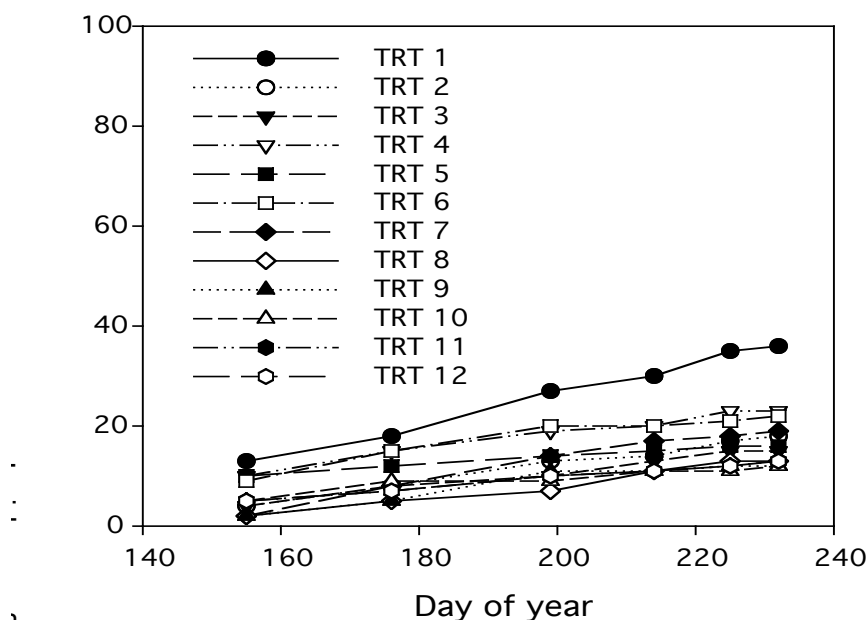
Figure 1. Disease incidence progress curves of Stewart's disease of corn for corn inbred (A632 Ht Block) plots at Crawfordsville, IA.
