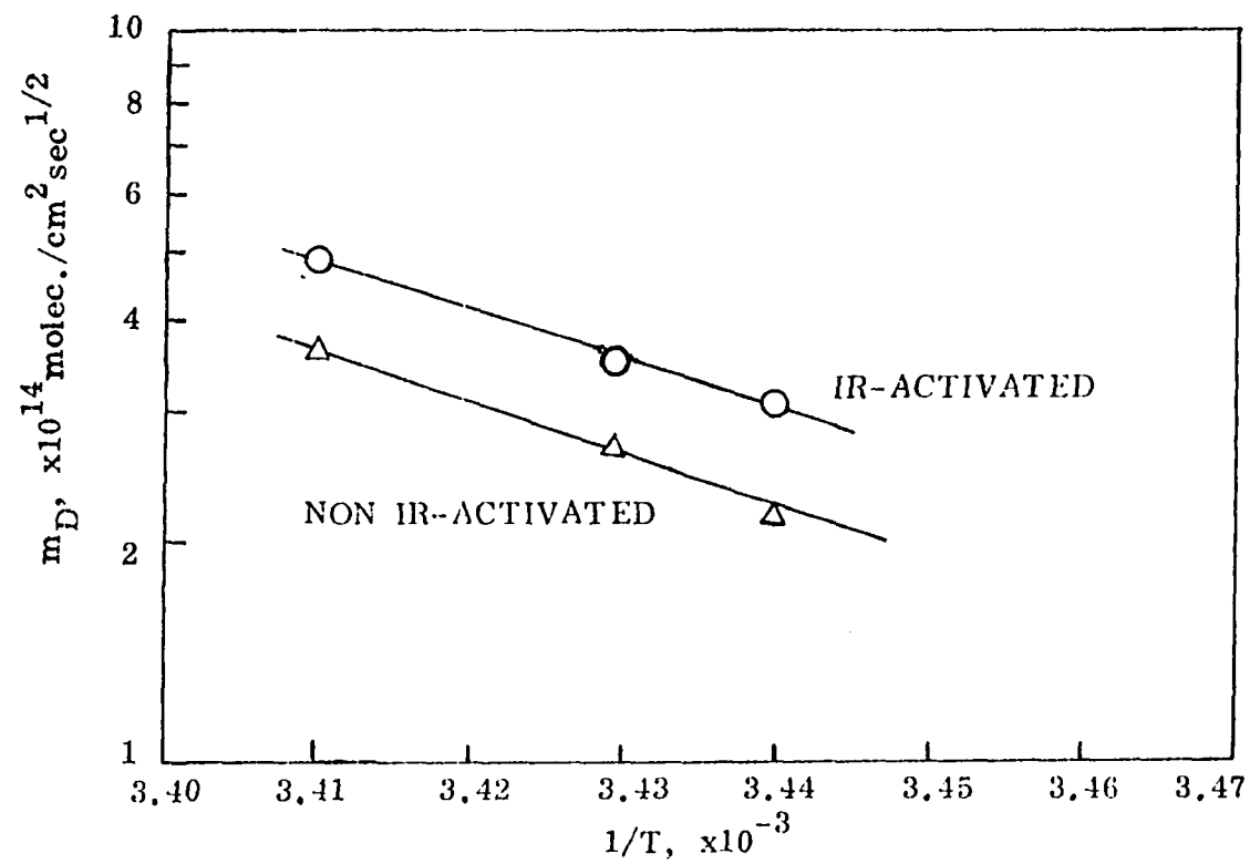
Figure 47. m_D versus reciprocal of temperature for water vapor adsorbed onto E-glass
