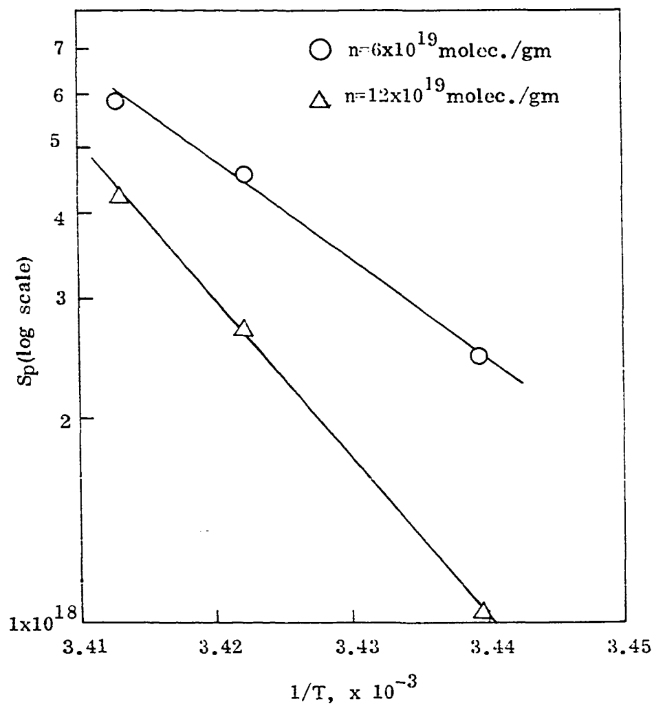
Figure 43. Dependence of the sticking probability of water vapor upon E-glass surface on temperature
