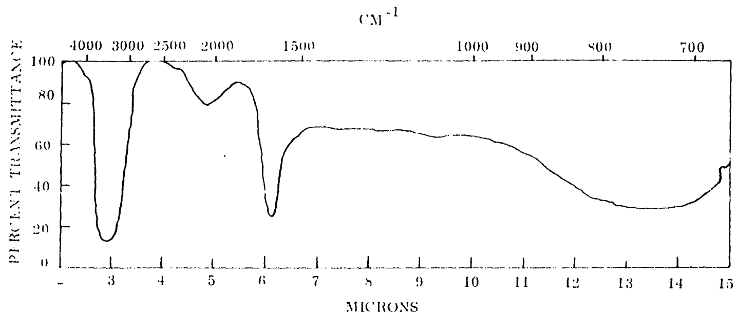
Figure 5. Qualitative analysis of the distilled water used by infrared spectroscopy
