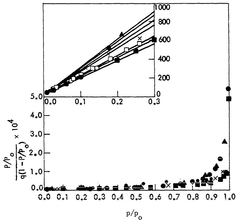
Figure 19. BET plots for water vapor adsorbed on E-glass
