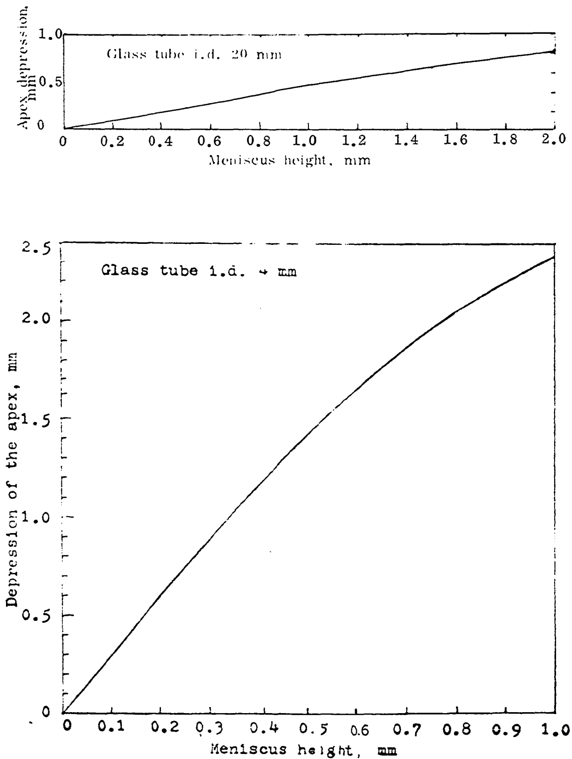
Figure 12. Capillary depression of the apex of a mercurial column in a glass tube
