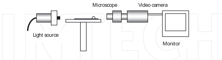
Figure 1. Contact angle measuring system
