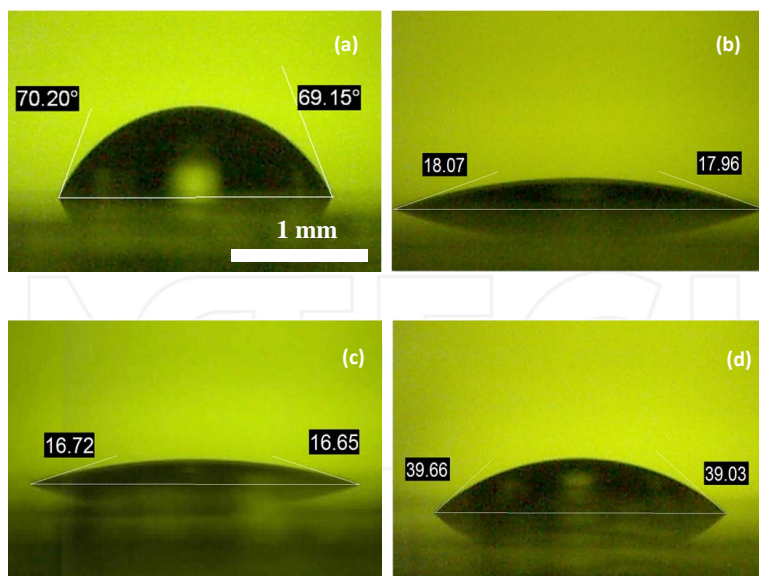
Figure 2. Contact angle images of (a) DI water droplet on non-treated PU film, (b) DI water droplet on 600sec UV-ozone treated PU film, (c) \text{CH}_2\text{I}_2 droplet on non-treated PU film, and (d) \text{CH}_2\text{I}_2 droplet on 600sec UV-ozone treated PU film
