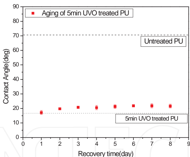
Figure 7. Change of the water static contact angle values versus aging time for polyurethane thin films after 5 minutes of UV ozone exposure
