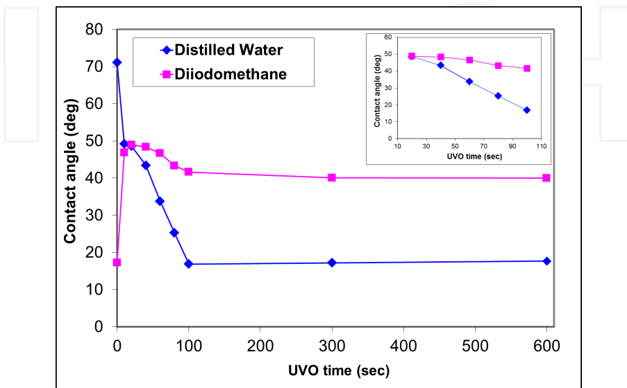
Figure 3. Contact angles of distilled water and diiodomethane on PU films (Insert shows the middle regime when UVO time is between 20 and 100 seconds)
