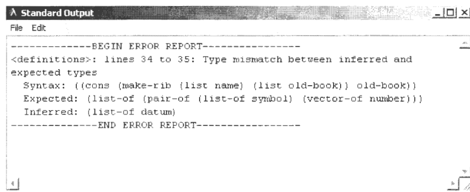
Figure 7.2 DrScheme Type Error Output
