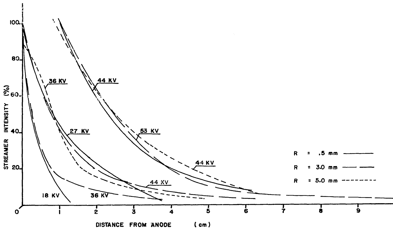
Figure 44. Comparison of streamer intensity decrease of various point radii and potentials.
