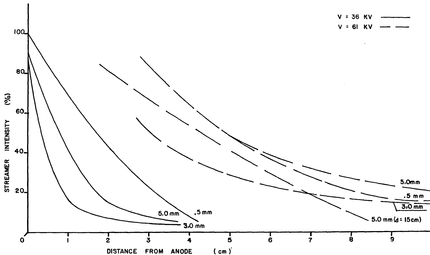
Figure 33. Comparison of streamer light intensities of various point radii at 44 KV and 61 KV.
