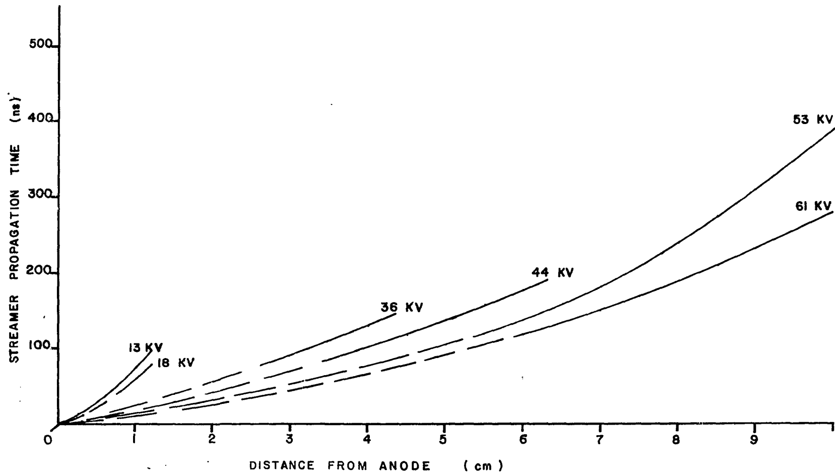
Figure 28a. Propagation time.
