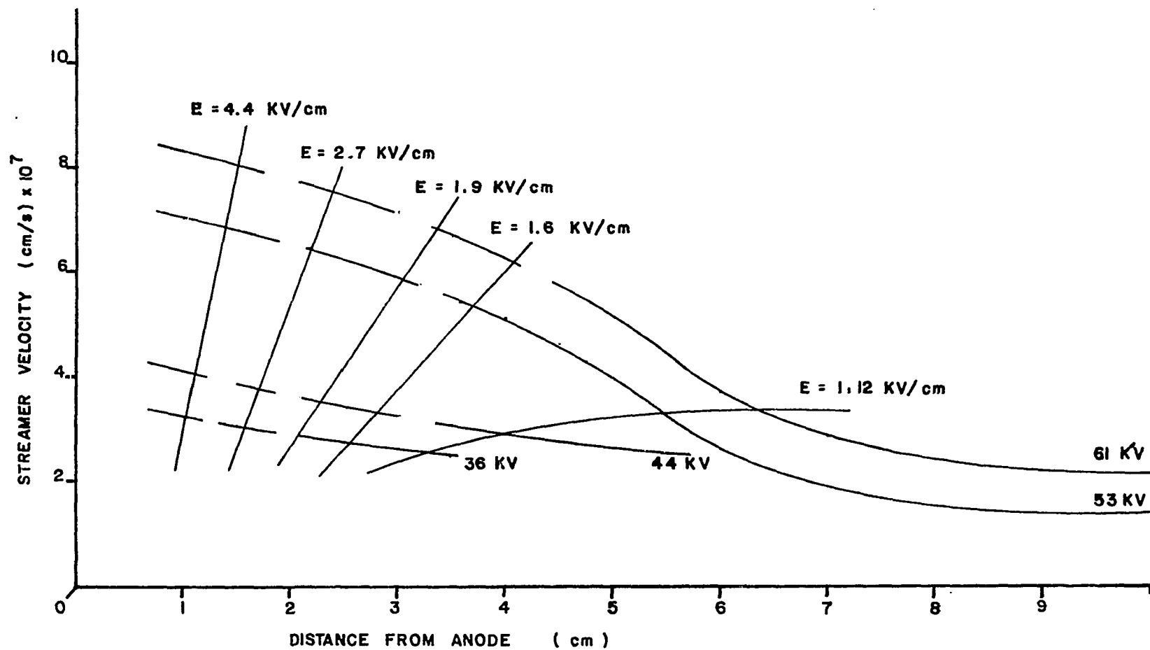
Figure 31a. Streamer velocity.
