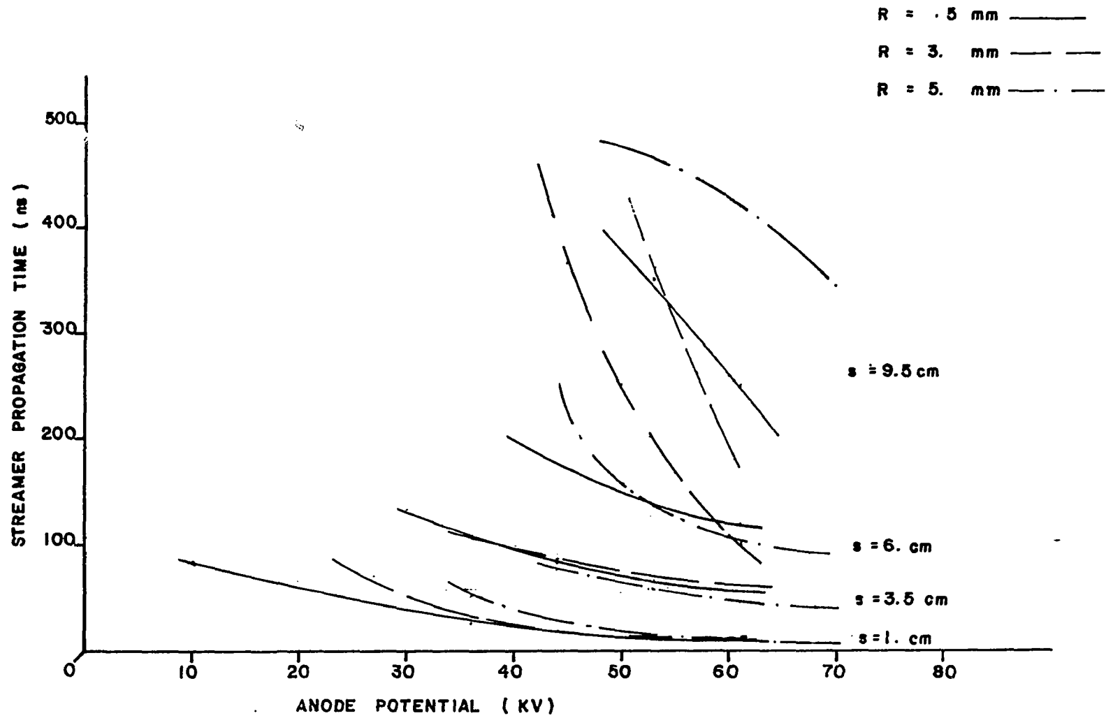
Figure 29. Propagation time versus potential at various locations in the gap.
