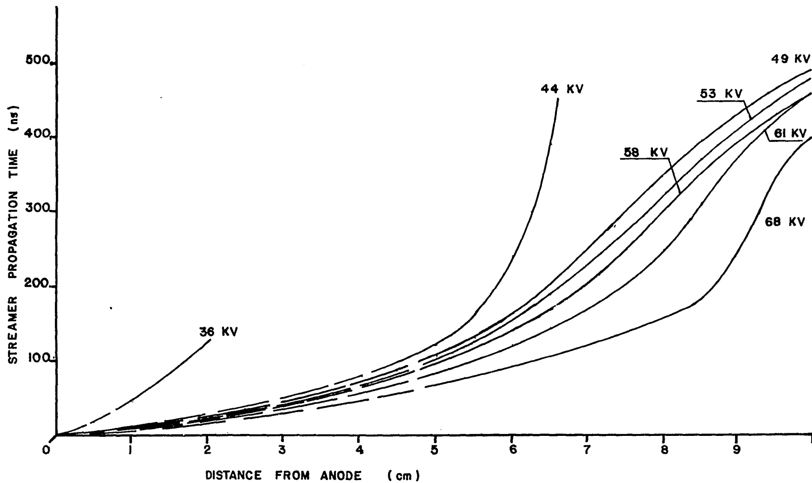
Figure 28c. Propagation time.
