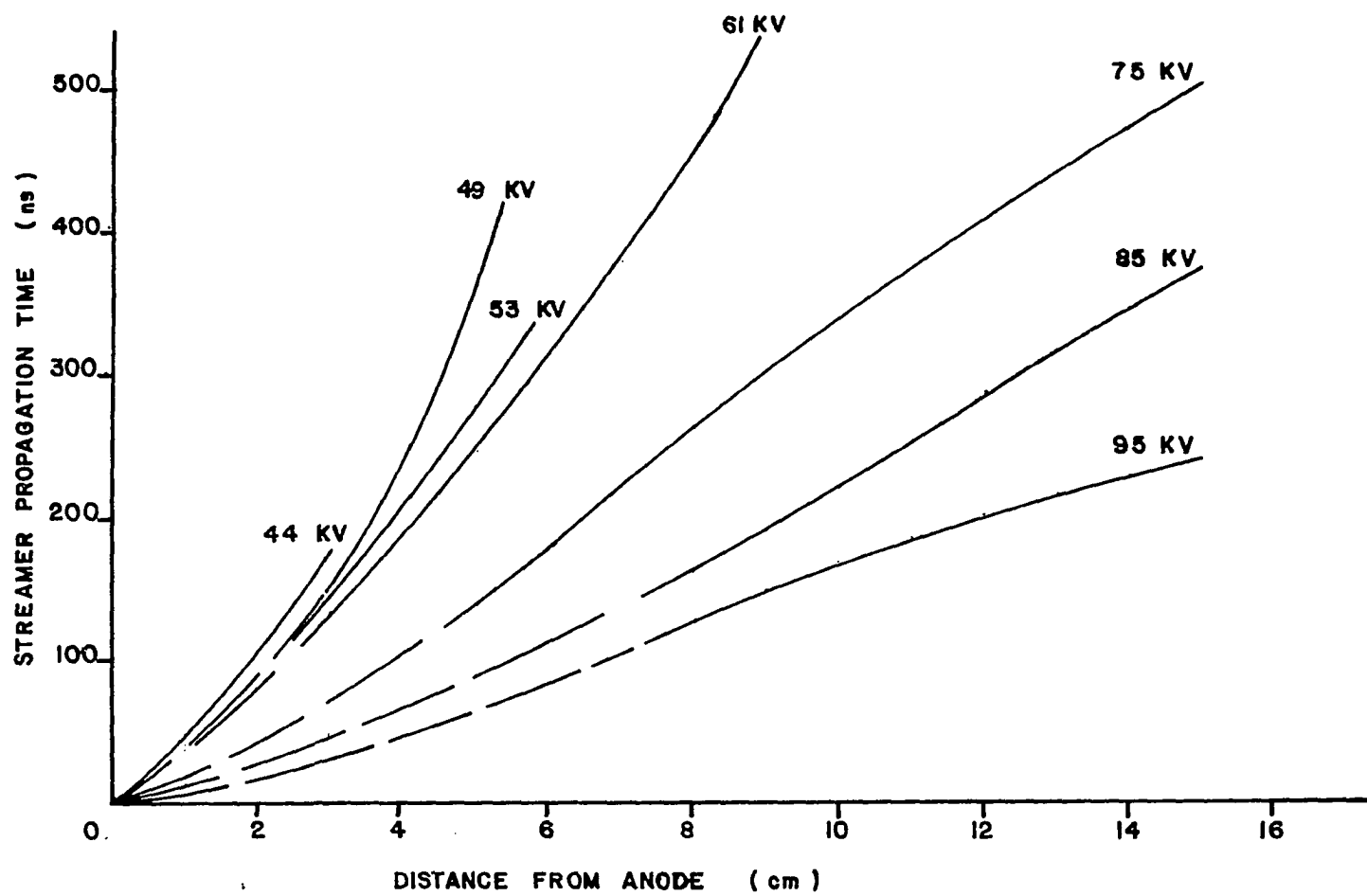
Figure 28d. Propagation time.
