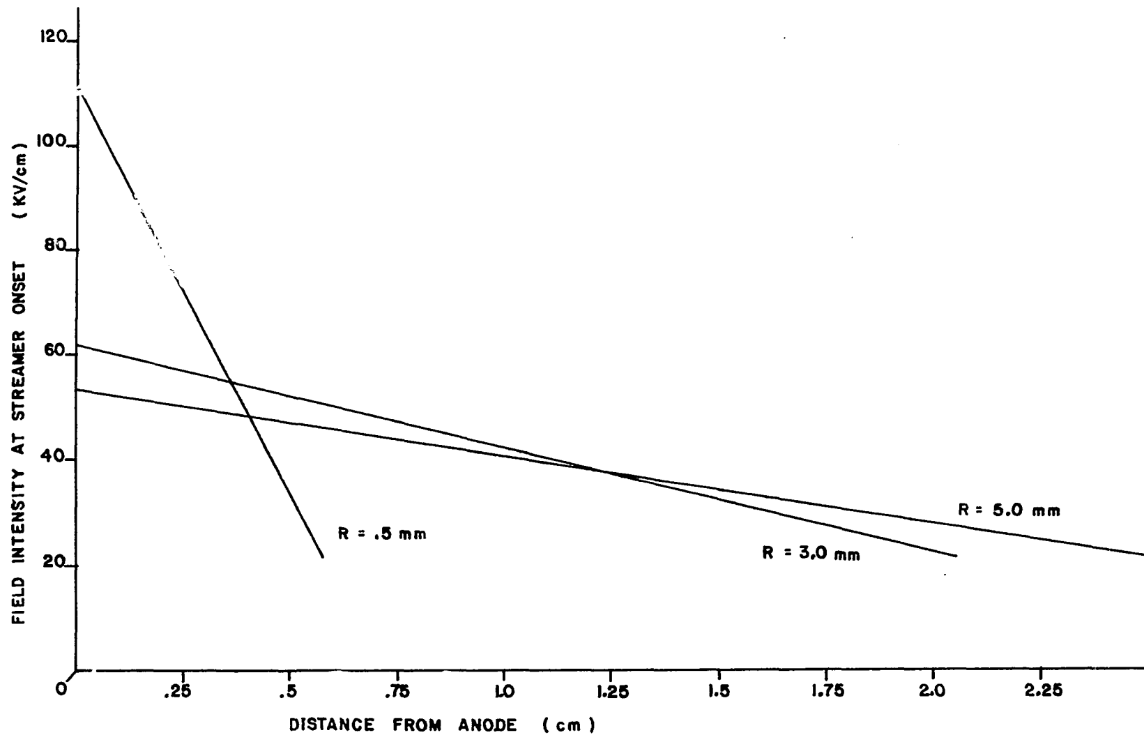
Figure 41. Field intensity and initial avalanche length for d = 10 cm and various point radii of streamer onset.
