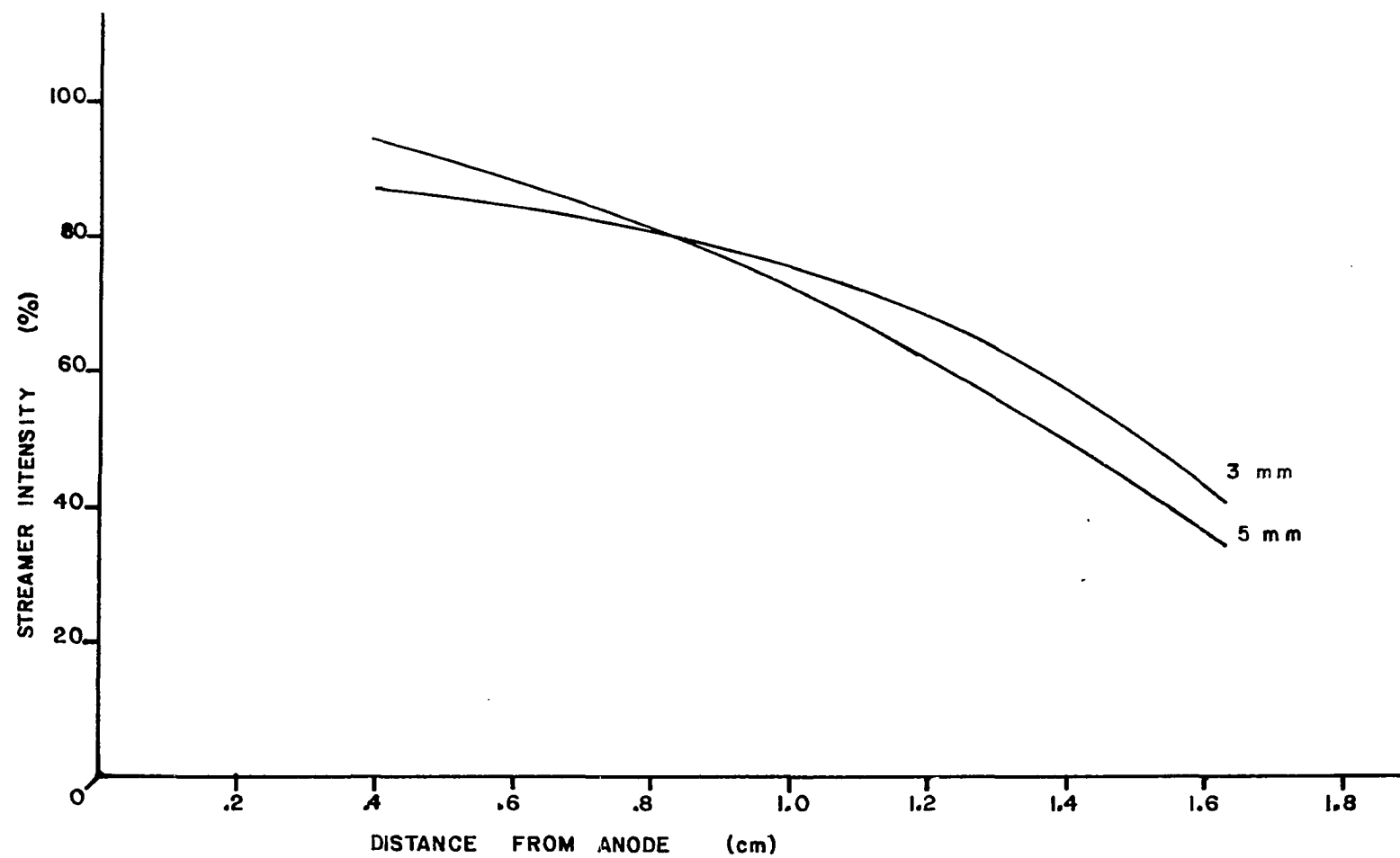
Figure 34. Streamer intensity in the anode region.
