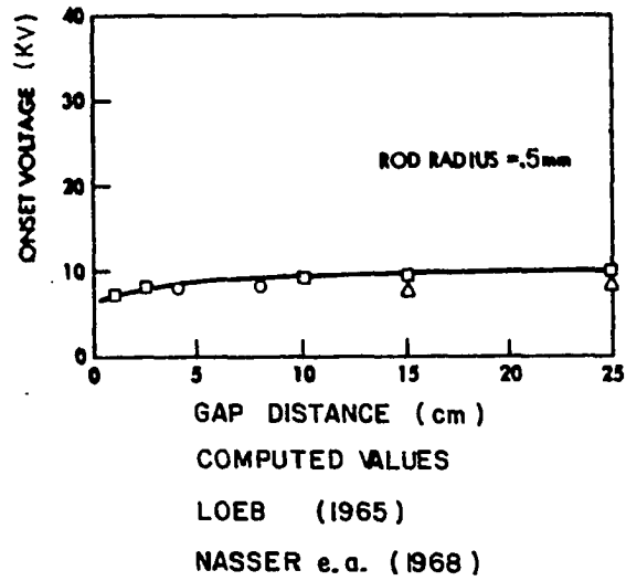
Figure 37. Comparison of computed and measured streamer onset potential.
