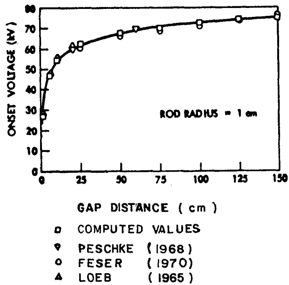
Figure 36. Comparison of computed and measured streamer onset potential.
