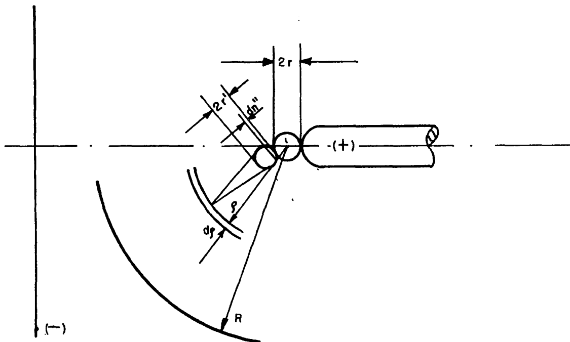
Figure 45. Critical avalanche of streamer onset.
