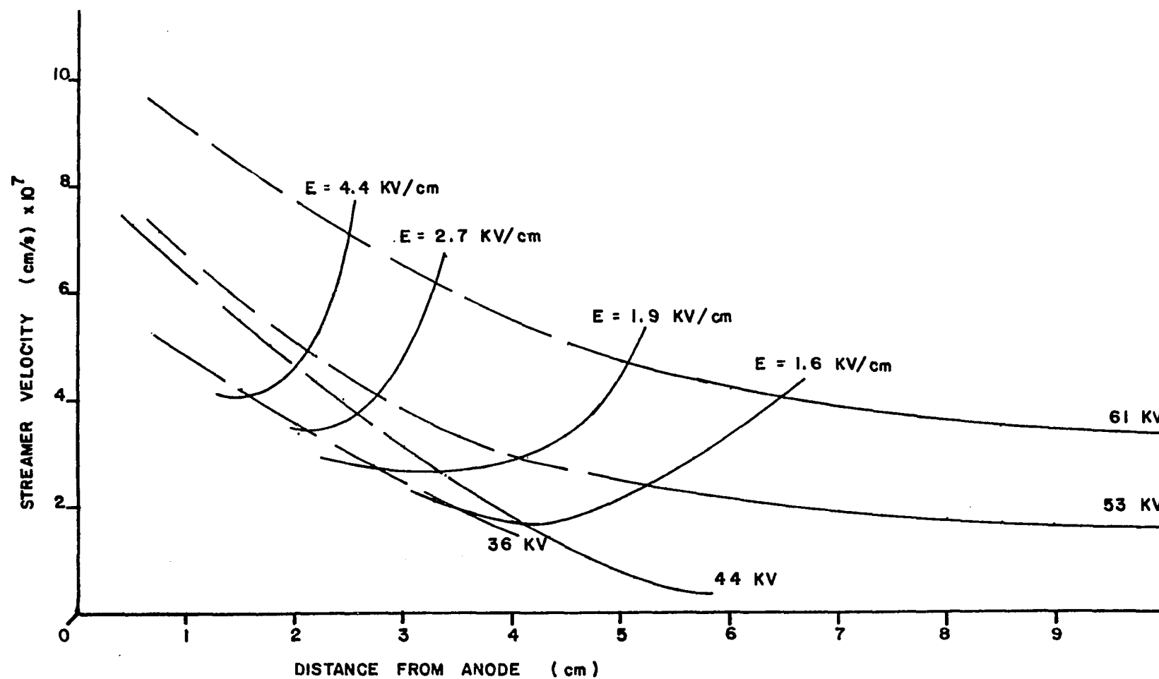
Figure 31b. Streamer velocity.
