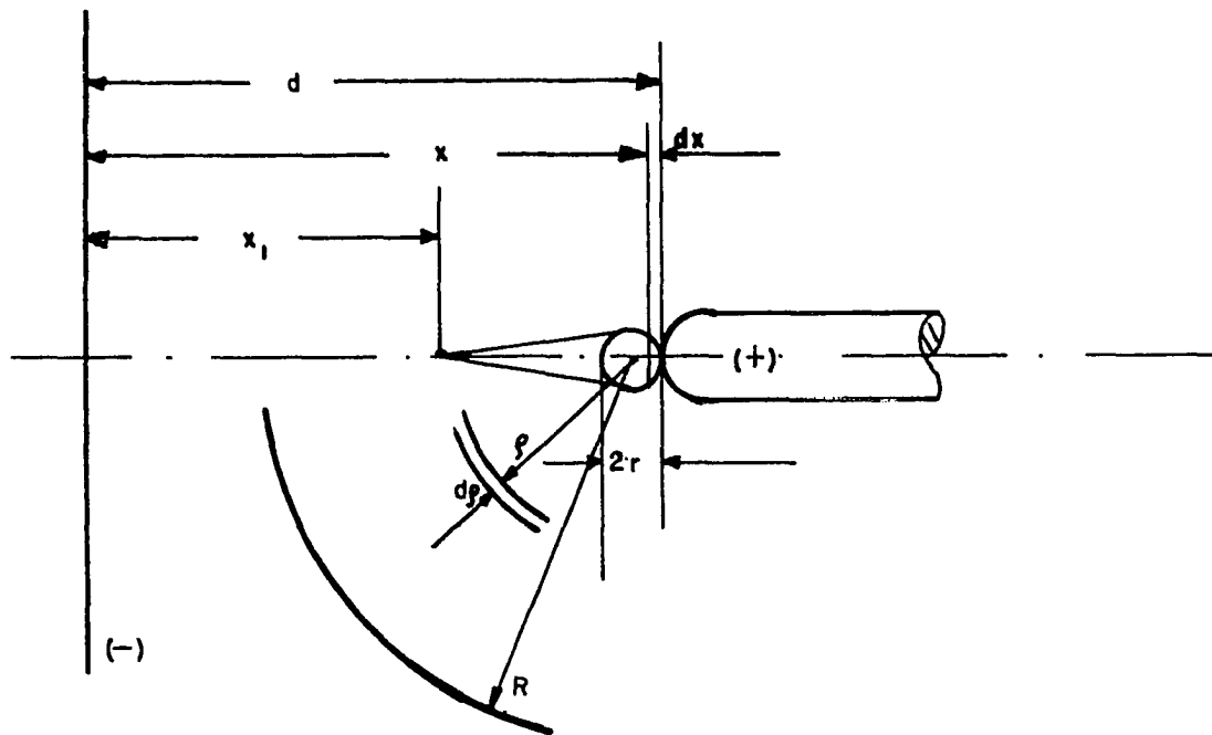
Figure 45. Critical avalanche of streamer onset.
