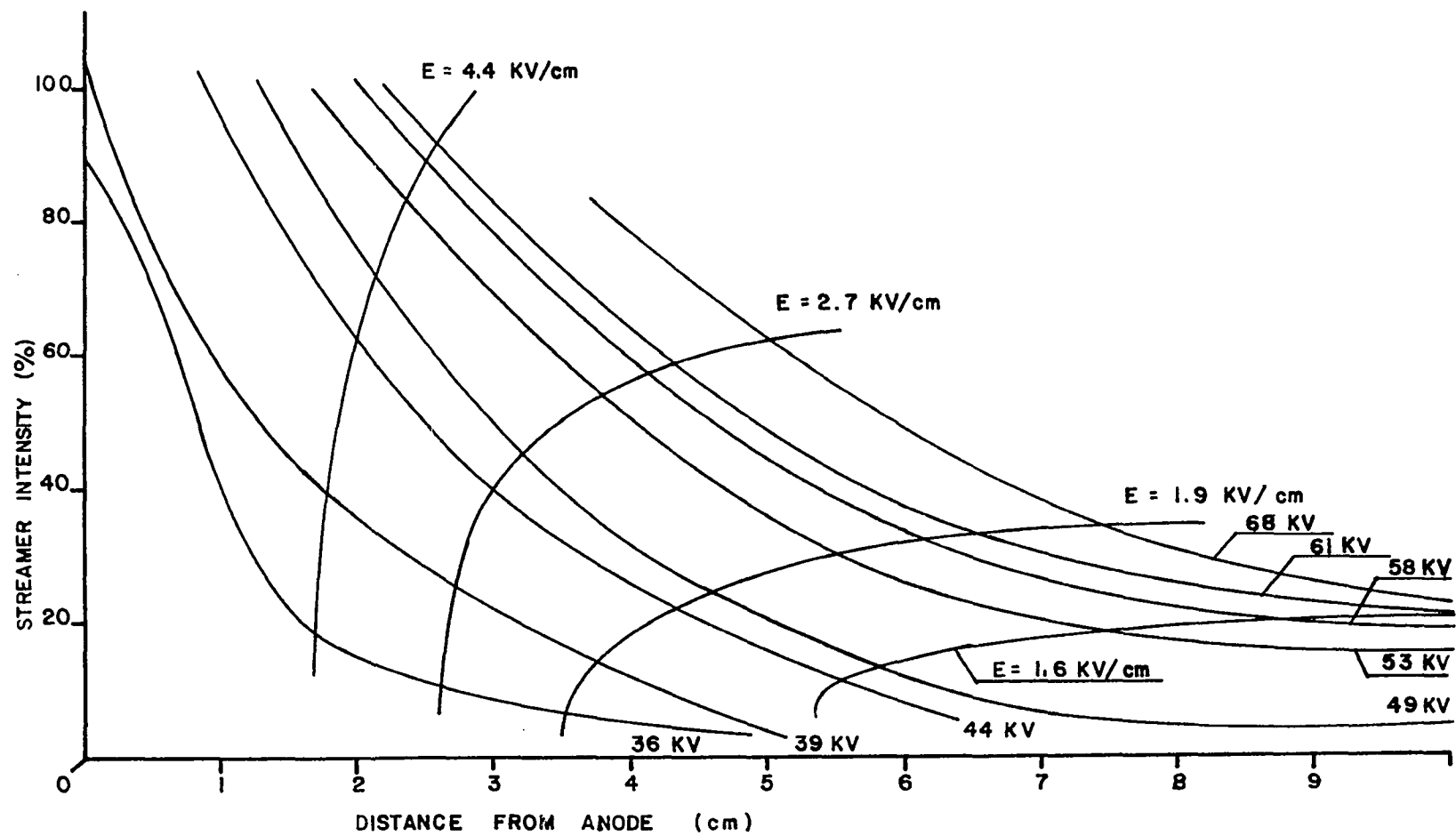
Figure 32c. Streamer intensity.
