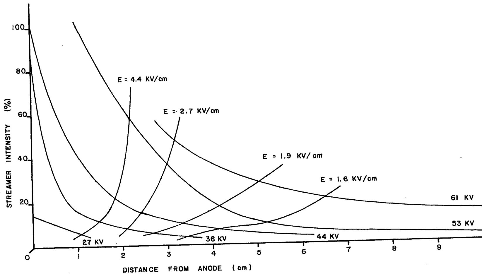
Figure 32b. Streamer intensity.
