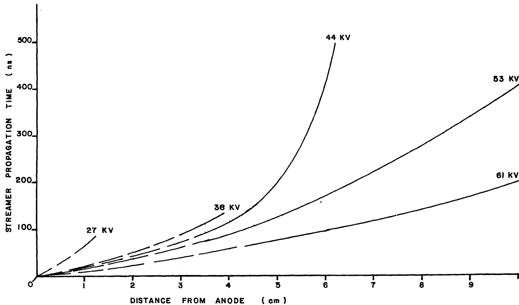
Figure 28b. Propagation time.
