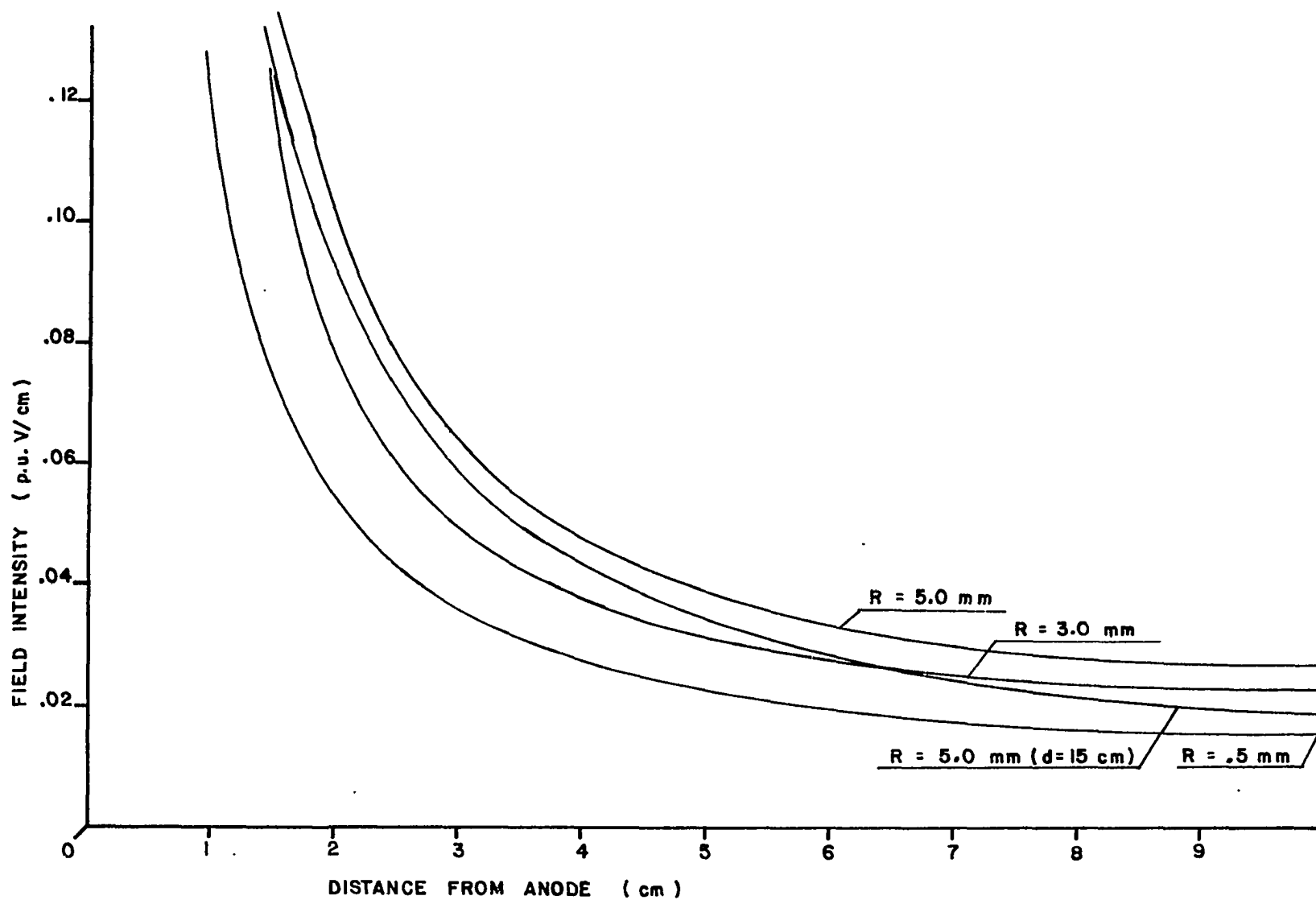
Figure 40b. Field distribution in the low field region for various point radii.
