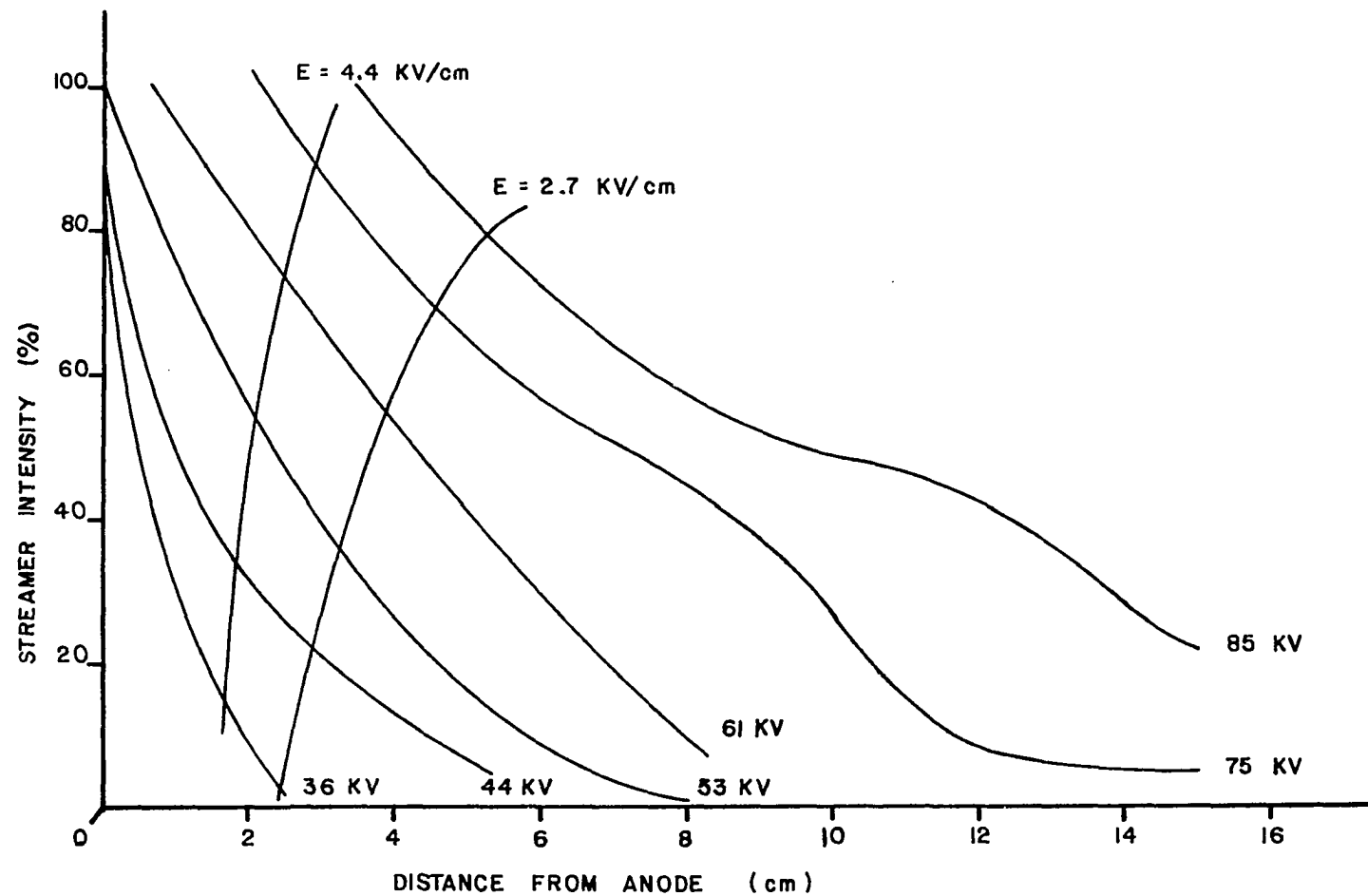
Figure 32d. Streamer intensity.
