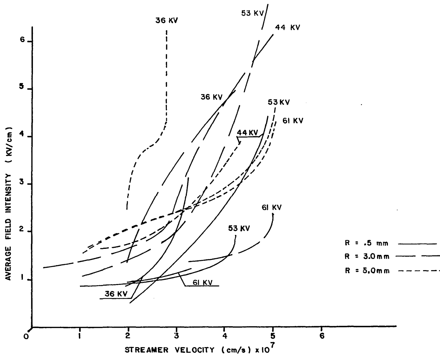
Figure 42. Field intensity streamer velocity for various point radii and potentials.
