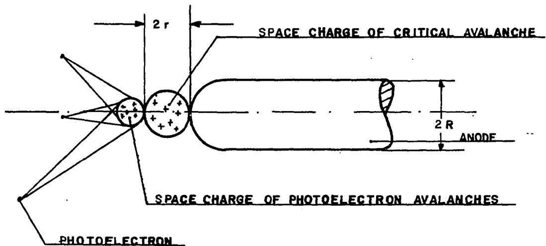
Figure 2. Criterion for streamer propagation.
