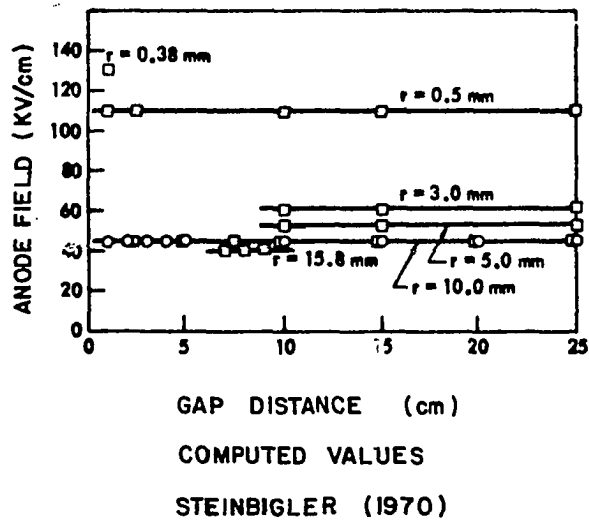
Figure 38. Comparison of computed and measured anode field intensity at streamer onset.
