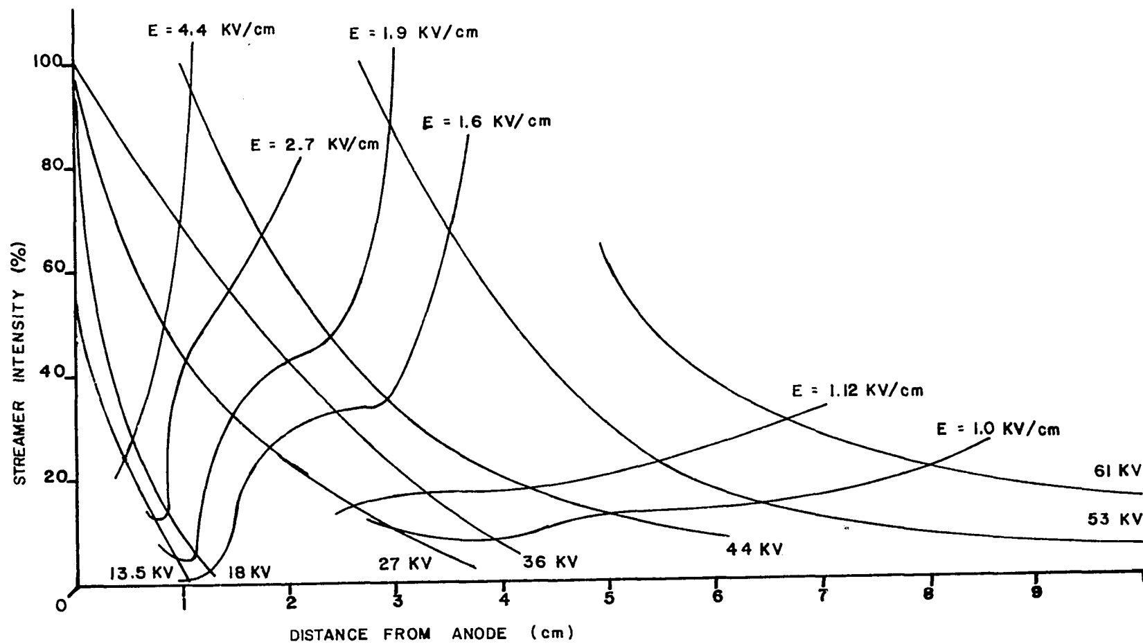
Figure 32a. Streamer intensity.
