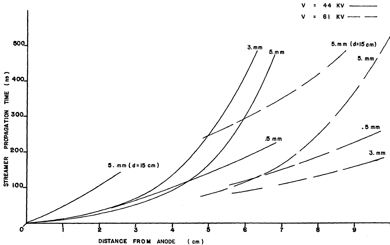
Figure 30. Propagation time of streamer for various point radii at 44 KV and 61 KV.
