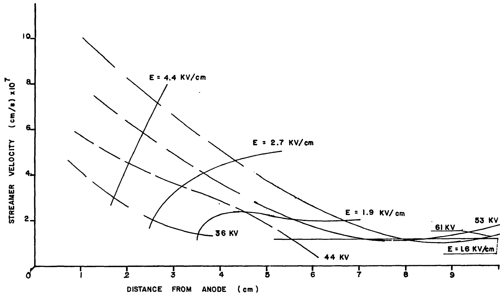
Figure 31c. Streamer velocity.
