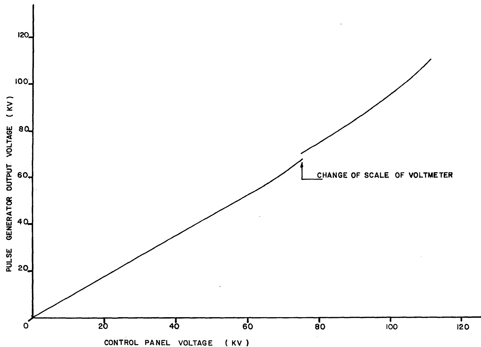
Figure 58. Calibration of the impulse generator.
