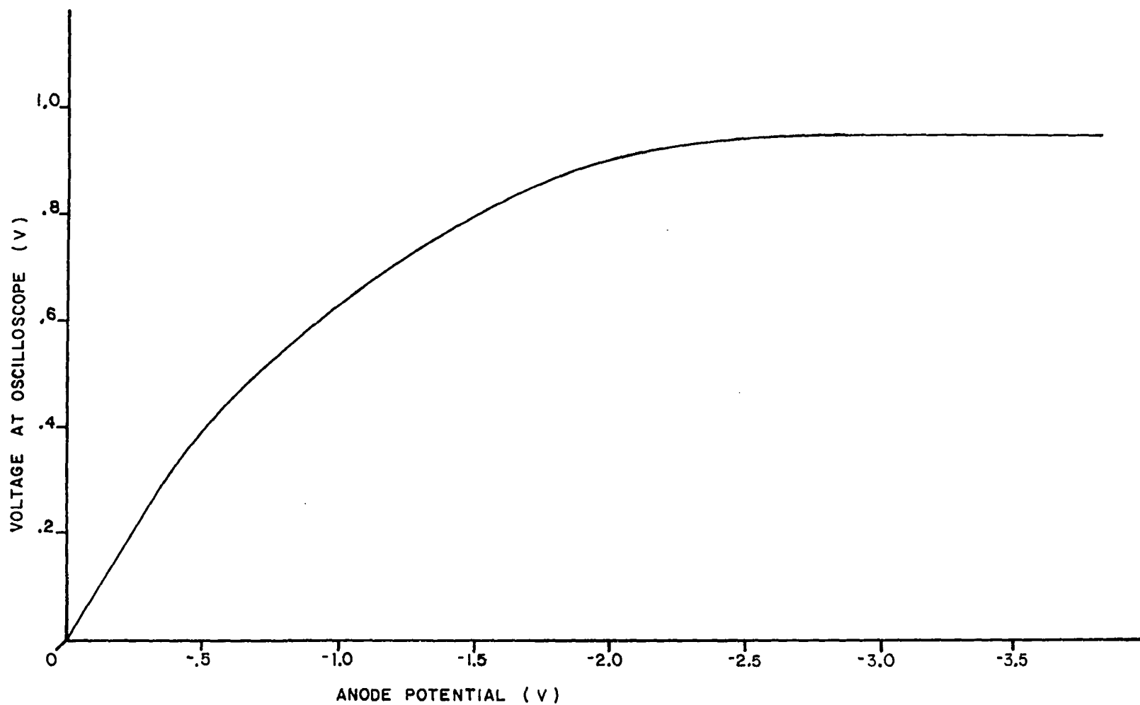
Figure 75. Calibration of the measuring circuit.
