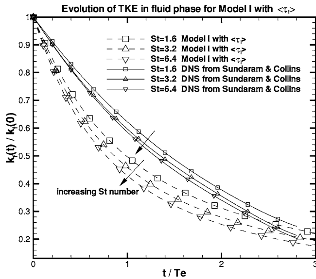
FIG. 6. Evolution of TKE in fluid phase from model I with the multiscale interaction time scale \langle \tau_i \rangle . Comparison of model results with DNS data.
