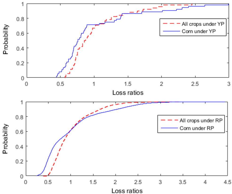
Figure 5. CDF of loss ratios for corn and for all crops under 85% coverage of YP or RP
