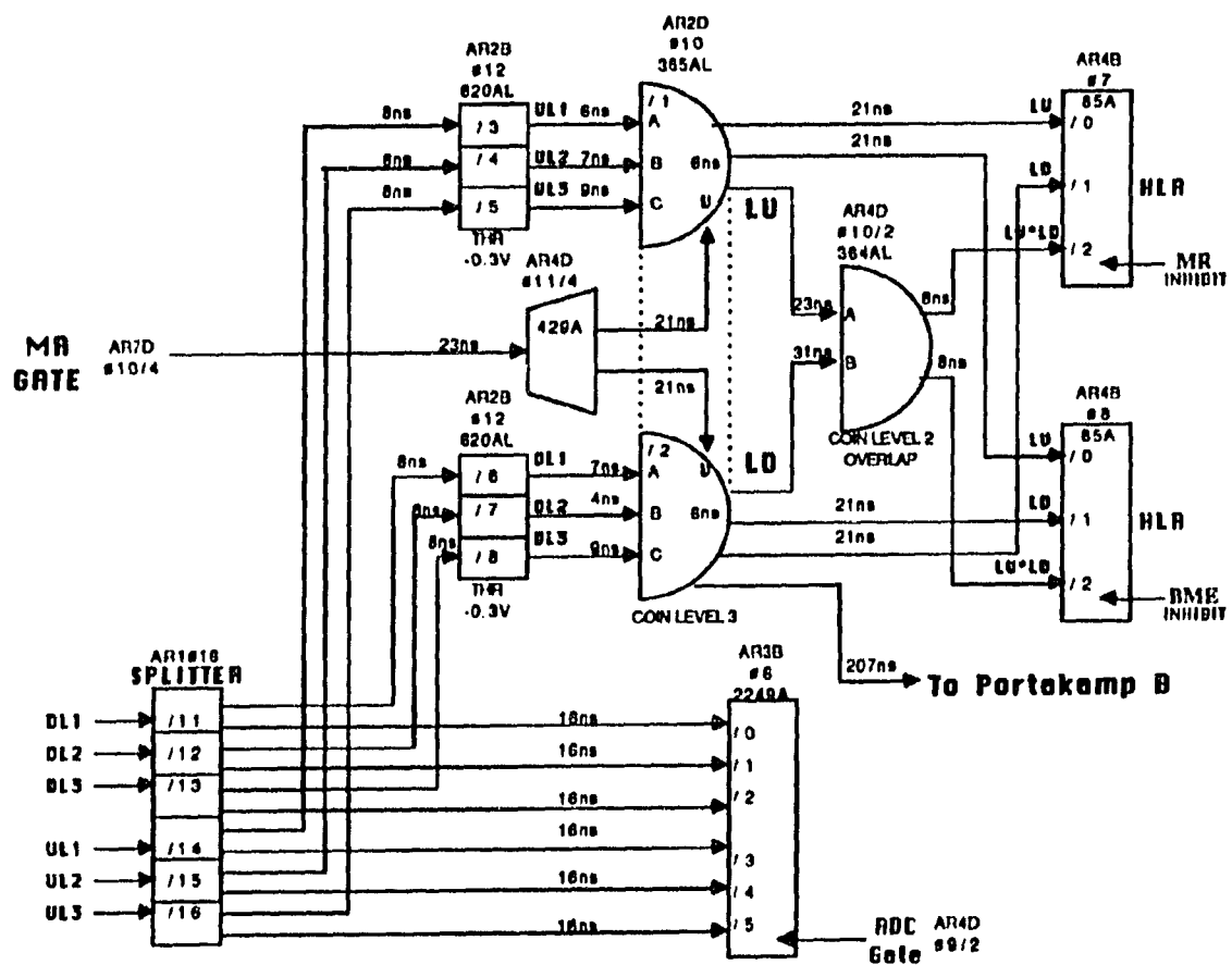
Figure A.10: Scaler inhibit and luminosity counters.
