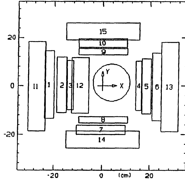
Figure 3.11: Projection of p \bar{p} counters on x-y plane.
