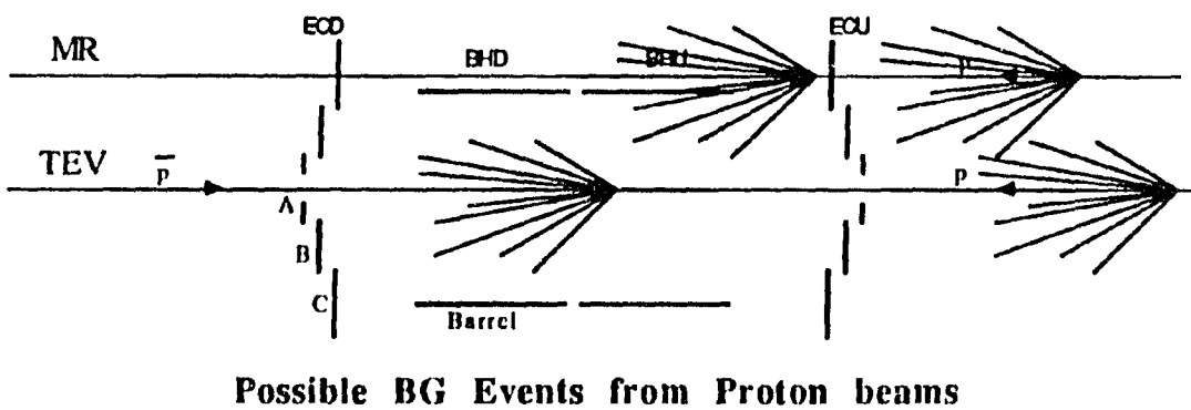
Figure 5.7: Sources of events.
