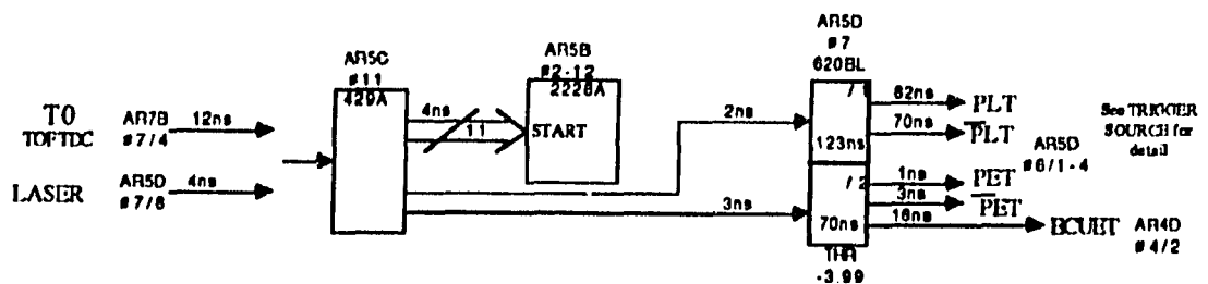
Figure A.7: Hodoscope and TOF.
