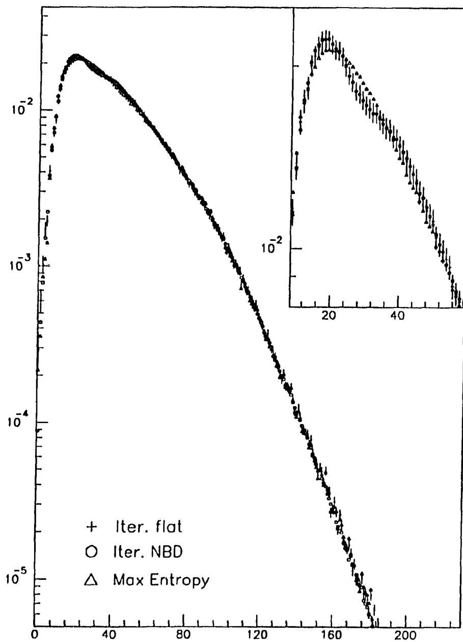
Figure 5.45: Reconstructed N_c(hodo) using maximum entropy and iteration methods. Before acceptance correction.
