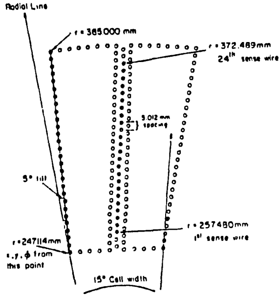
Figure 3.5: Cross section of a CTC supercell.
