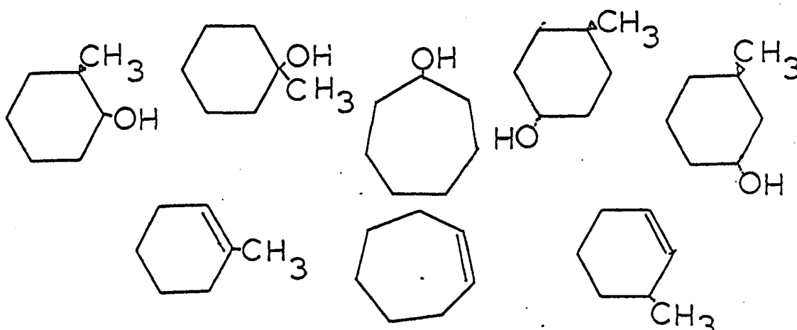
Figure 11. Products from the acid-catalyzed ring opening of norcarane
