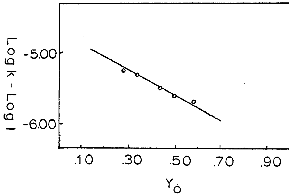
Figure 25. The hydrolysis of 3-menthene
