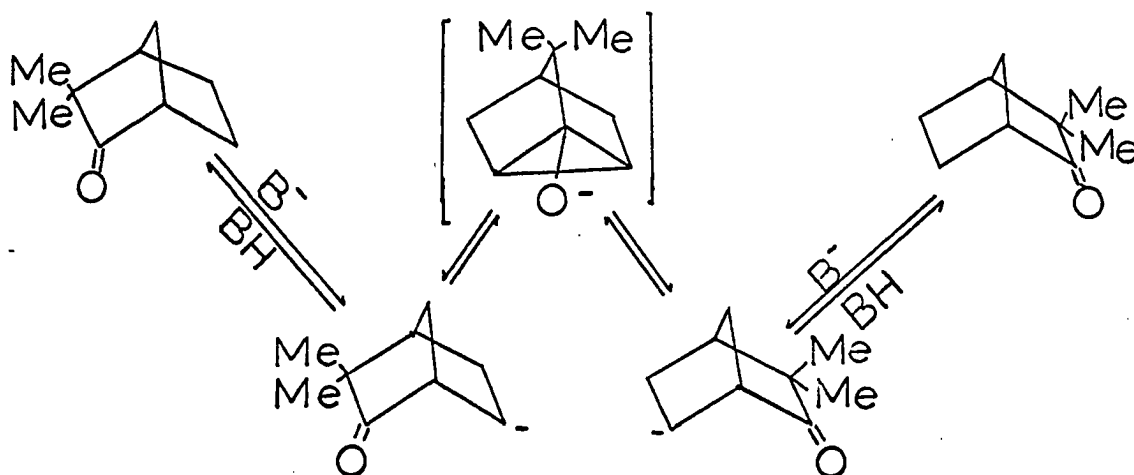
Figure 7. Nickon's postulated cyclopropanol anion intermediate in the racimization of camphinilone
