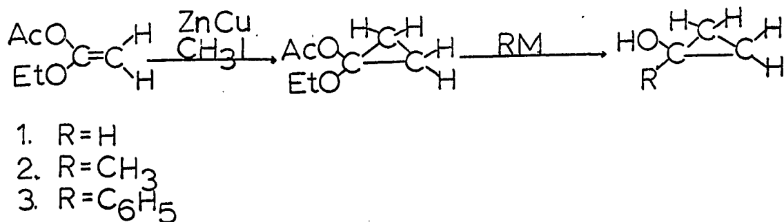
Figure 4. The synthesis of cyclopropanols by use of zinc-copper couple
