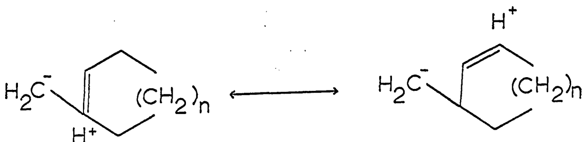
Figure 10. Most probable ground state resonance forms for bicyclo[n.1.0]alkanes
