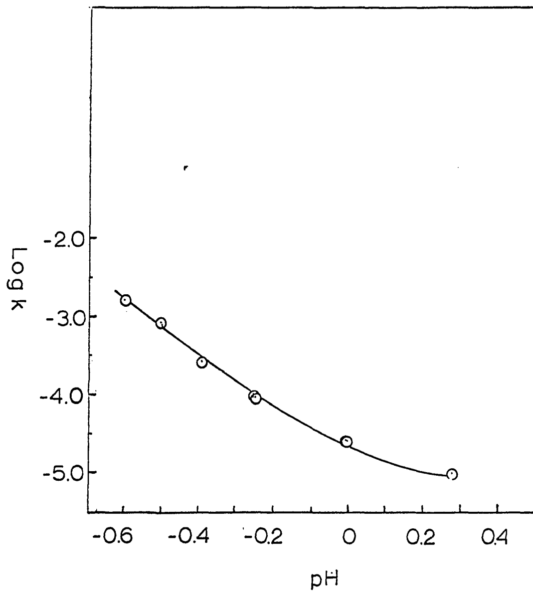
Figure 19. Plot of \log k vs. \text{pH} for the ring opening of 1-p-methylphenylcyclopropanol
