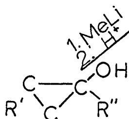
Figure 2. Eiler's method of preparation of substituted cyclopropanols
