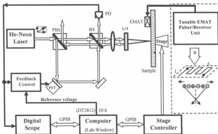
Figure 1. Schematic diagram of the EMAT generation and laser detection system.
