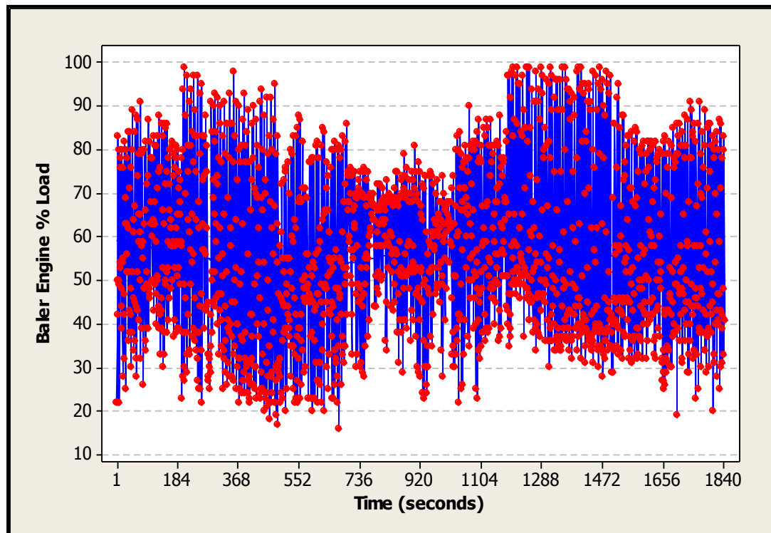
Figure 6-9: Time-series plot for 12 row collection stover collection for the towed baler. As the baler requires more power to operate from the higher rates of stover being collected the engine load will approach 100% but also consistently stay higher on the cyclical load because of the higher loads on the baler.
