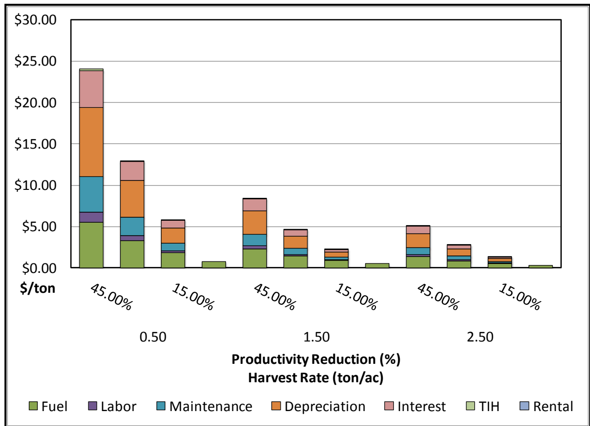
Figure 7-8: Total cost per ton for the combine to harvest stover broken down into seven cost categories for analysis based upon cost data from the ASABE D497 standard and current machine prices.
