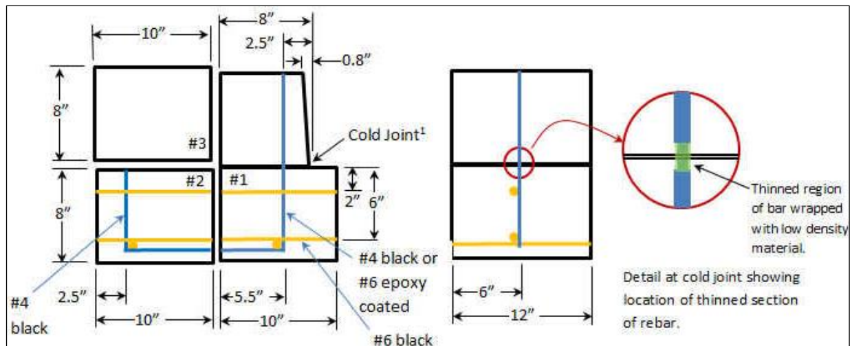
Figure 3. Configuration of test specimens
