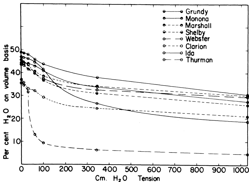
Fig. 6. Moisture retention curves from 0 cm to 1 atmosphere of tension for the eight Iowa soils upon which infiltration measurements were made with the rainfall simulator.
