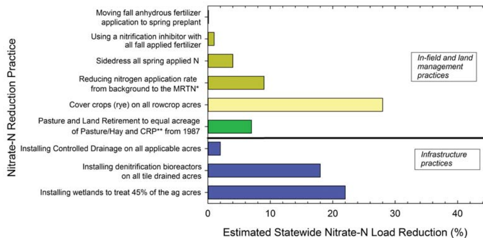
Estimated statewide nitrate-N reductions in Iowa with maximum practical implementation of individual practices.
