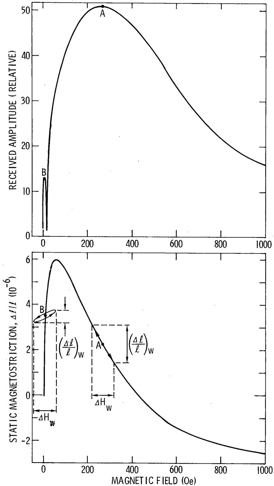
Fig. 3. Measured transducer efficiency and magnetostriction vs magnetic field in 1018 steel.
