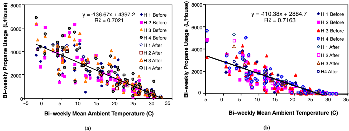
Figure 6. Relationship of bi-weekly propane fuel use of broiler houses to bi-weekly mean outside temperature for Northwest Arkansas area. Solid legends depict those before renovation and hollow legends depict those after renovation. (a) Weeks 1 and 2; (b) Weeks 3 and 4.
