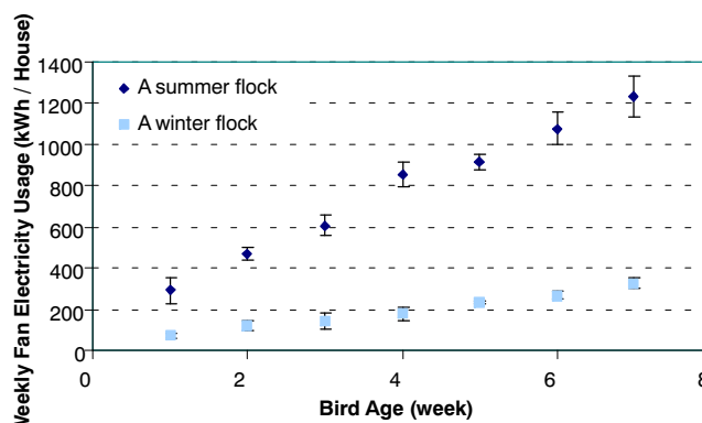
Figure 3. Sample weekly electricity use by ventilation fans of broiler houses during winter or summer.
