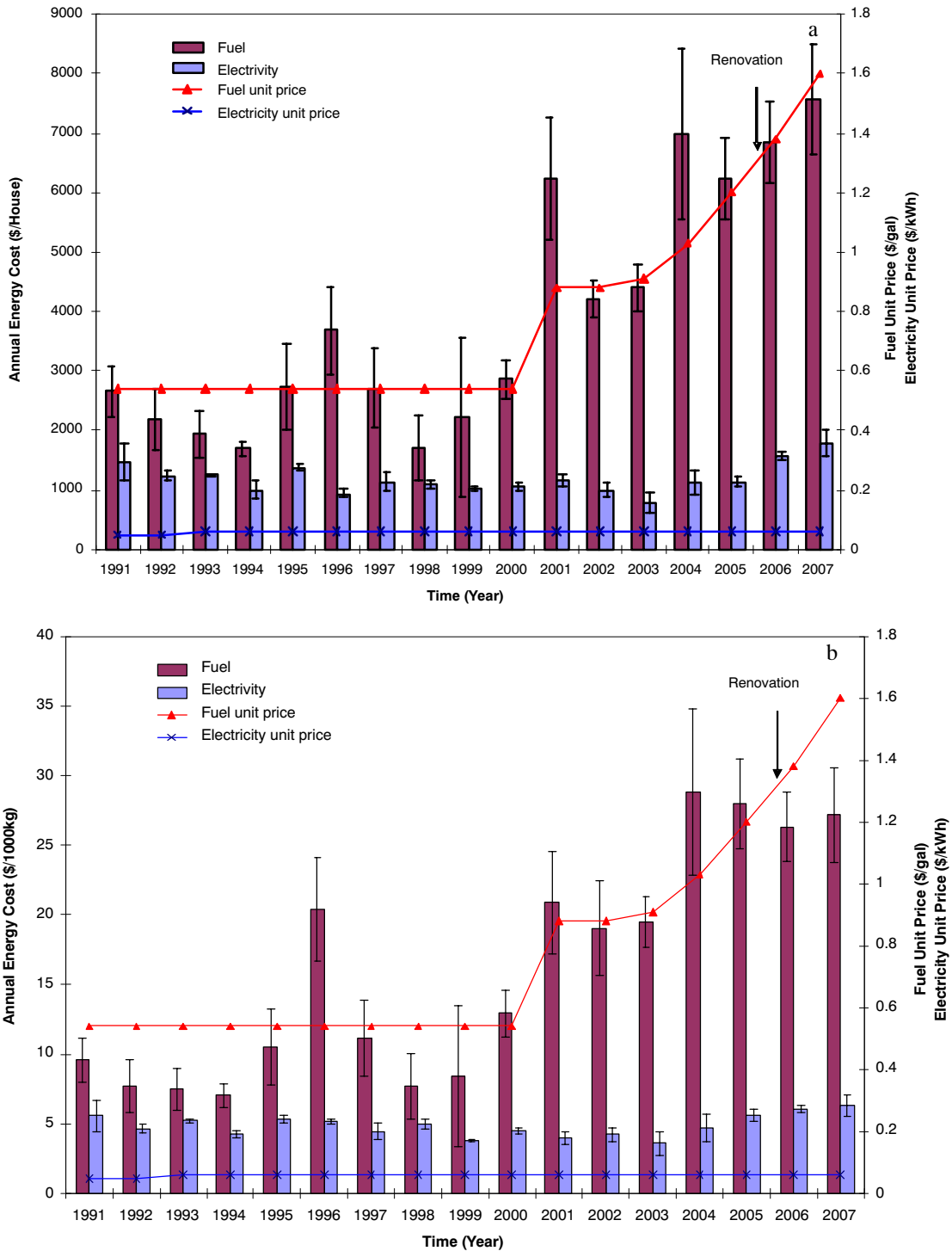
Figure 7. Annual costs of propane and electricity and the actual local energy charges (a) averaged per house; (b) average per 1000 kg live market weight. Error bars represent the standard deviation of the four houses.
