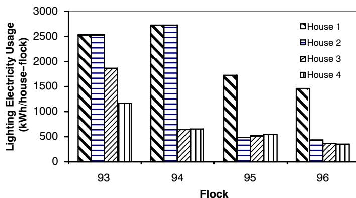
Figure 4. Lighting electricity usage for four broiler flocks (May 2007-Feb. 2008) from four houses using various types of light bulbs (table 2). House 1: incandescent; House 2: incandescent for flocks 93 and 94, dimmable fluorescent for flocks 95 and 96; House 3: cold cathode fluorescent light with 2700 Kelvin for flock 93 and 4000 Kelvin for flocks 94 to 96; House 4: cold cathode fluorescent light with 4000 Kelvin.
