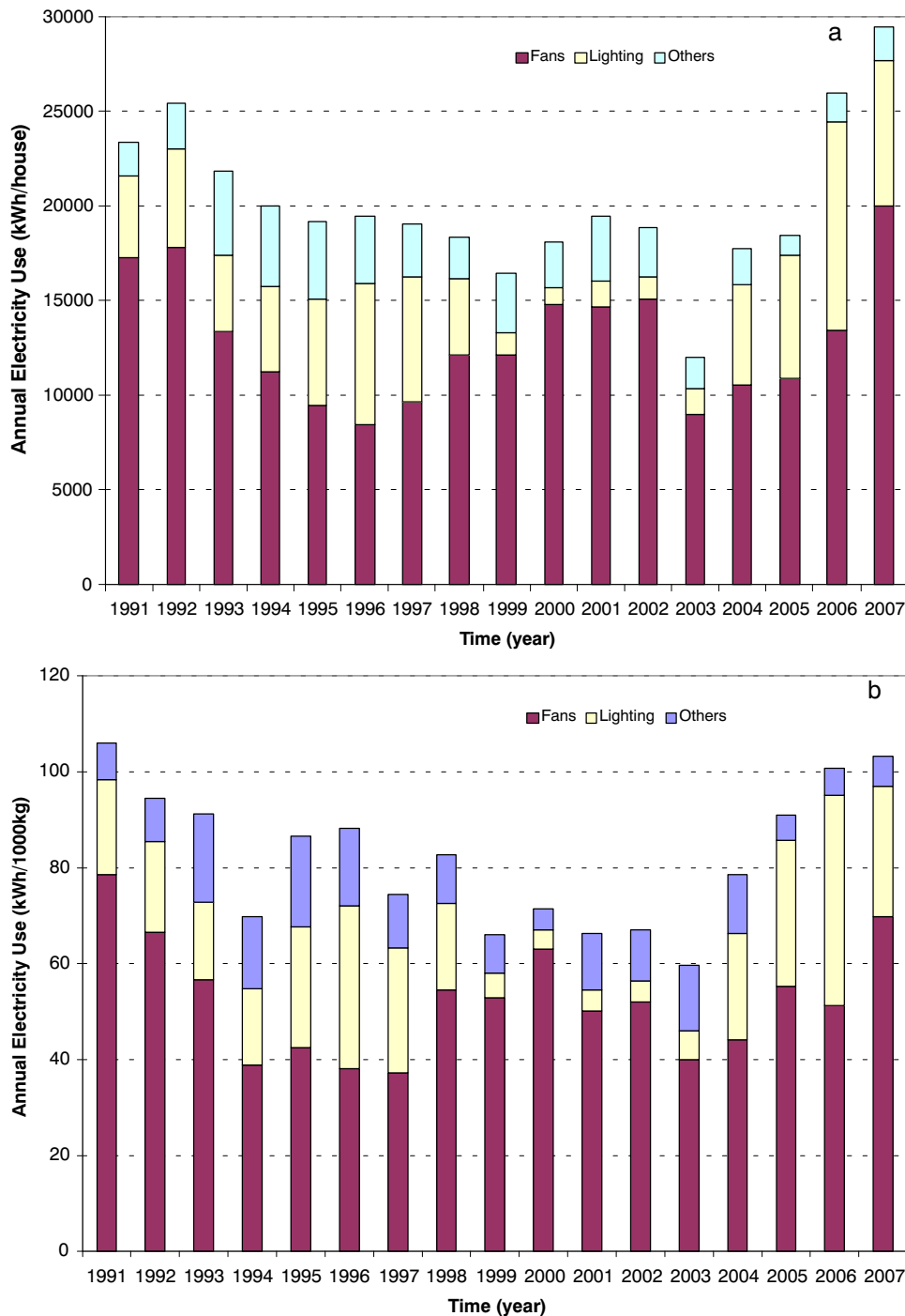
Figure 2. Annual electricity usage by fans, lighting and others. (a) usage by house; (b) usage by 1000-kg market live bird weight.
