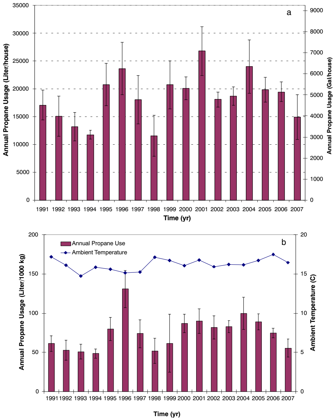
Figure 5. Annual propane usage and correspondent annual average outside temperatures (a) per house; (b) per 1000 kg market live weight. Error bars represent the standard deviation of the four houses.
