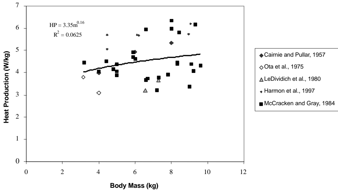
Figure 3. Swine heat production data for early-weaned pigs with a mass ( m ) of less than 10 kg from five independent studies from 1957 through 1997. Regression model was not significant ( P = 0.125 ). Data used in this analysis were originally reported in references 1, 3, 5, 7, and 15 as defined in Appendix A.
