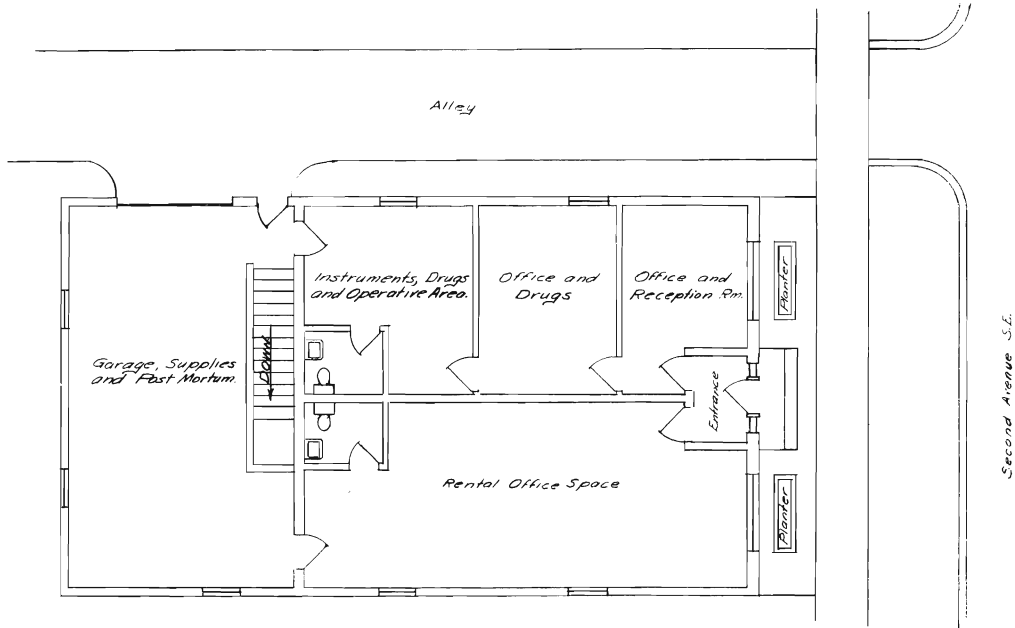
BELMOND VETERINARY CLINIC FLOOR PLAN Scale 1"=8'-0"
