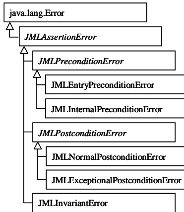
Figure 3: A part of the exception hierarchy for JML runtime assertion violations.
