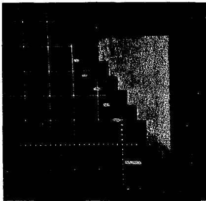
Figure 6. A B-scan image of a stepped sample compared with its optical image. The small steps are 5 mm wide with 8 mm distance between them.
