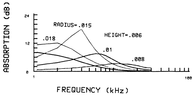
Figure 5. Absorption vs frequency for a rubber disc height of 6.0 mm. for holes of varying radii. Note the maximum in absorption for a hole of .015 meters and a hole height of .006 meters. All dimension are in meters.
