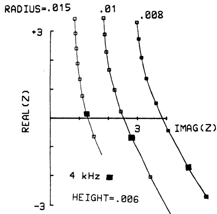
Figure 6. The impedance plane for an absorber with different radii and a rubber disk height of 6.0 mm. The large black square is a frequency marker at 4 kHz. Spacing between square markers is 2 kHz and all dimensions are in meters.
