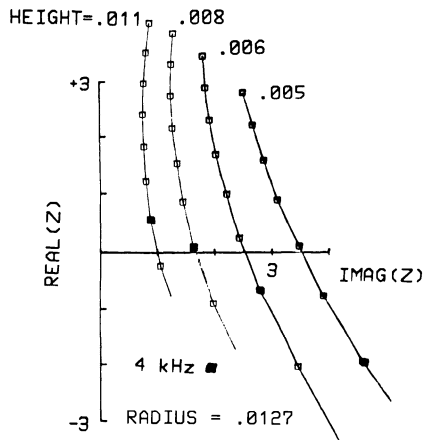
Figure 8. The impedance plane for absorbers with a hole diameters of 2.54 cm and different hole heights. All dimensions are in meters.
