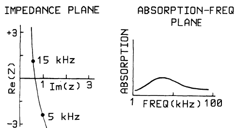
Figure 4. The relationship between the impedance plane the the absorption-frequency plane. The curve in the impedance plane crosses the abscissa at the resonant frequency while the absorpction-frequency plane shows a maximum in absorption at that frequency.
