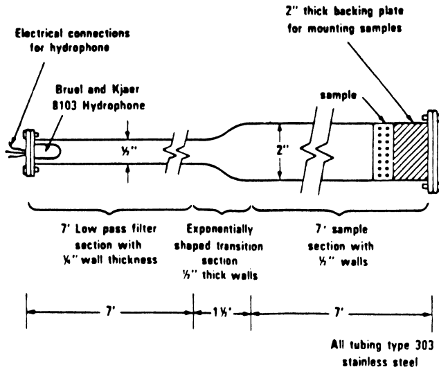
Figure 2. The NSWC guided wave tube. The small diameter section permits operation to 60 kHz.
