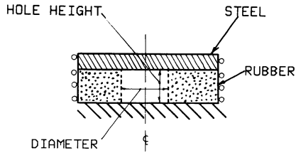
Figure 1. The axisymmetric absorber. The steel disk was 6.0 mm thick.
