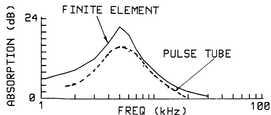
Figure 3. A comparison between panel data and guided wave tube data.
