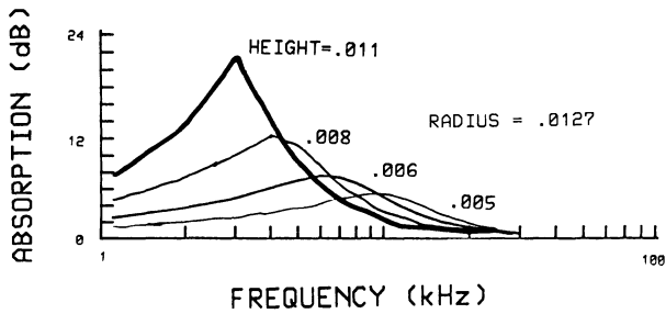
Figure 7. Absorption vs frequency for absorbers with a hole diameter of 2.54 cm and different hole heights. All dimensions are in meters.
