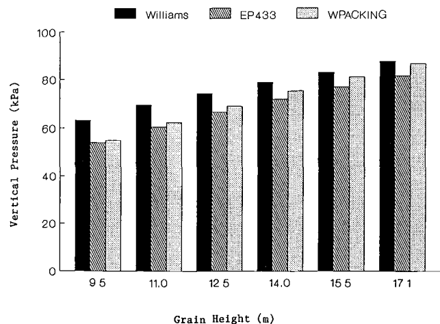
Figure 7—Vertical pressures in a 12.8 m (42 ft) diameter corrugated-walled grain bin storing corn [WPACKING- k=0.45 , u=0.34 , and w=720 \text{ kg/m}^3 ( 45 \text{ lb/ft}^3 ); EP433- k=0.5 , u=0.37 , and w=775 \text{ kg/m}^3 ( 48.4 \text{ lb/ft}^3 ); EP433- k=0.5 , u=0.317 , and w=775 \text{ kg/m}^3 ( 48.4 \text{ lb/ft}^3 )].
