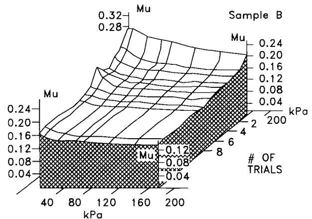
Figure 3—Variation in the coefficient of friction of wheat on galvanized steel as a function of lateral pressure and the number of trials (Thompson et al., 1988).
