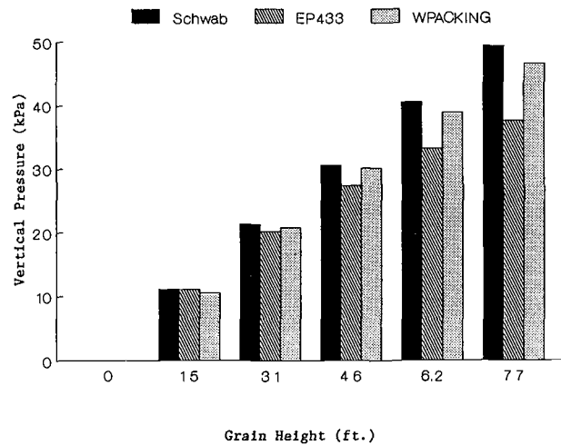
Figure 4—Vertical pressures in a 4.08 m (13.4 ft) diameter smooth-walled grain bin storing soft red winter wheat with a height-to-diameter ratio of H/d=1.8 [WPACKING- k=0.42 , u=0.14 , and w=724 kg/m^3 (45.2 lb/ft^3 ); EP433- k=0.5 , u=0.3 and, w=834 kg/m^3 (52 lb/ft^3 )].
