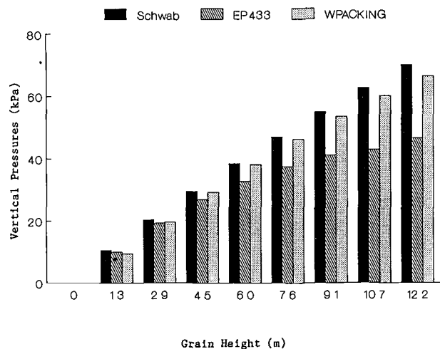
Figure 5—Vertical pressures in a 5.08 m (13.4 ft) diameter smooth-walled grain bin storing soft red winter wheat with a height-to-diameter ratio H/d=3.0 [WPACKING- k=0.42 , u=0.14 , and w=724 kg/m^3 (45.2 lb/ft^3 ); EP433- k=0.5 , u=0.3 , and w=834 kg/m^3 (52 lb/ft^3 )].
