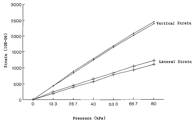
Figure 2—Vertical and lateral strains of soft red winter wheat within a grain pressure apparatus using a diaphragm pressure cell.
