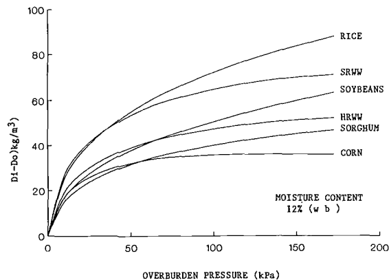
Figure 1—Variation in bulk density of six whole grains for a moisture content (wb) of 12% (Thompson et al., 1987).
