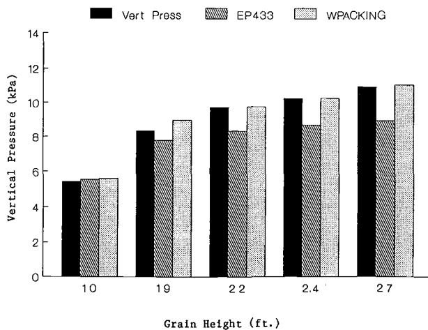
Figure 6—Vertical pressures in a 0.91 m (3 ft) diameter corrugated-walled model grain bin storing soft red winter wheat [WPACKING- k=0.421 , u=0.27 , and w=724 \text{ kg/m}^3 ( 45.2 \text{ lb/ft}^3 ); EP433- k=0.5 , u=0.37 , and w=834 \text{ kg/m}^3 ( 52 \text{ lb/ft}^3 )].
