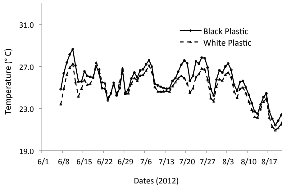
Figure 1. Soil temperature 4 in. under soil in plastic mulch treatments.
