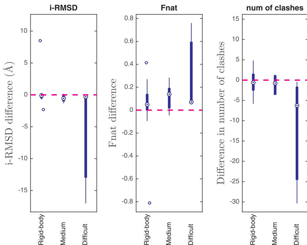
Figure 3: Performance differences between CA-CA-guided docking and superimposition over the BM4 dimer cases with rigid-body, medium, large conformational changes. A negative i-RMSD difference means that the top four CA-CA models of a docking case have a lower average i-RMSD than its top four superimposed models. Likewise, the positive difference in Fnat and the negative difference in the number of clashes mean that the top four CA-CA models are better than the top four superimposed models. 'Rigid-body', 'Medium' and 'Difficult' correspond to low, medium and large conformational changes, respectively [21]. The superiority of CA-CA-guided docking over superimposition becomes increasingly clear as the amount of conformational changes on binding increases.
