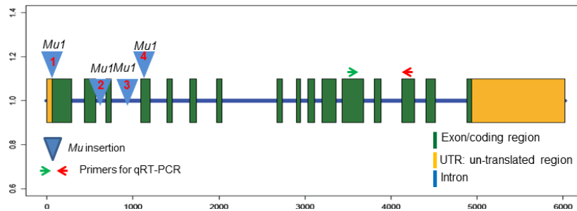
Figure 4. Sequence analysis of bm4-Mu alleles.
