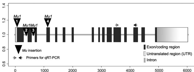
Figure 4. Sequence analysis of bm4-Mu alleles. Mu insertions in bm4 were detected in alleles: (1) bm4-Mu 13-7033E , (2) bm4-Mu 11-8050D , (3) bm4-Mu 13-7029B , and (4) bm4-Mu 13-7064E .
