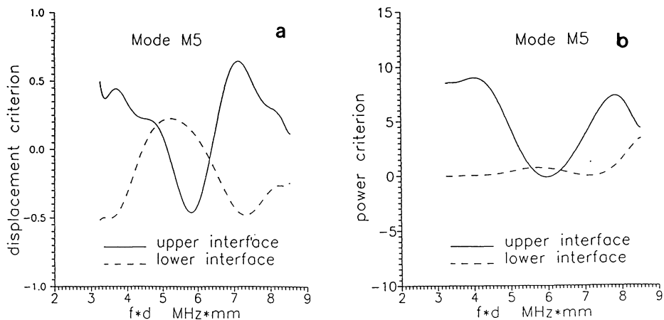
Fig. 4. Displacement (a) and power (b) criteria for the fifth mode and given range of fd .
