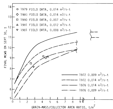
Fig. 11— Final average grain moisture vs. grain-mass/collector-area (central Iowa).
