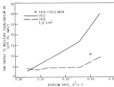
Fig. 7—Electrical energy for fan operation per unit grain mass vs. airflow rate for a grain-mass/collector-area ratio of 1.2 t/m 2 (central Iowa).
