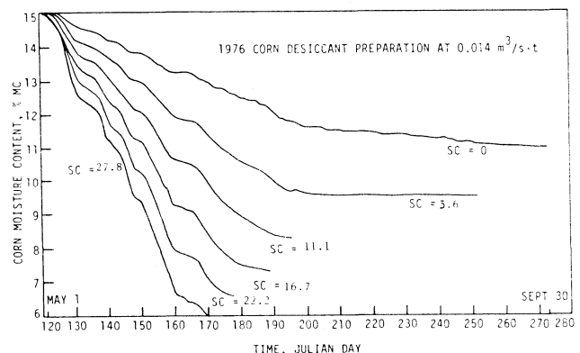
Fig. 2—Corn moisture content vs. time for 1976 solar corn desiccant preparation in central Iowa.
