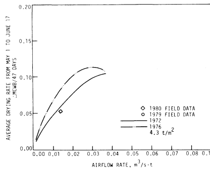
Fig. 4—Average drying rate vs. airflow rate for a grain-mass/collector-area ratio of 4.3 t/m 2 (central Iowa).
