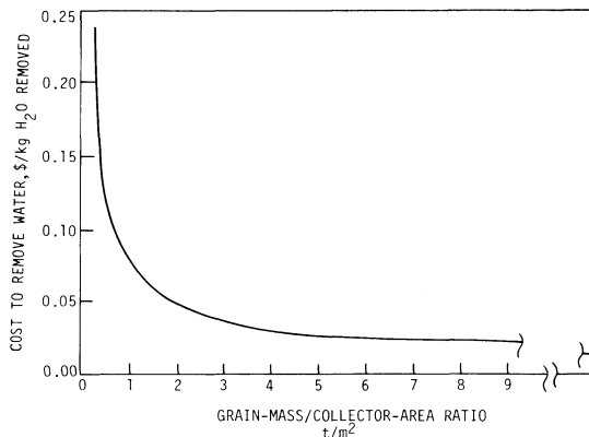
Fig. 13— Cost to remove water vs. grain-mass/collector-area. Airflow rate: 0.014 m 3 /s·t (central Iowa).
