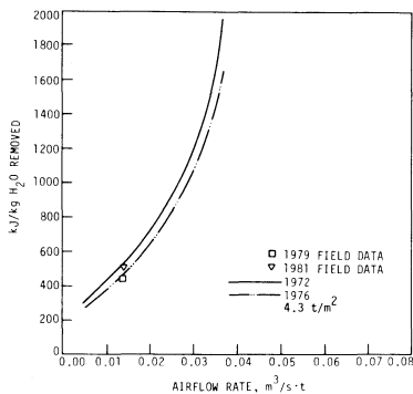
Fig. 10— Electrical energy for fan operation per unit of water removed for a grain-mass/collector-area ratio of 4.3 t/m 2 . Grain depth = 4.6 m (central Iowa).
