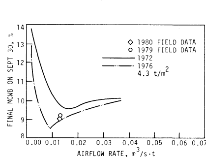
Fig. 6—Final grain moisture content vs. airflow rate for grain-mass/collector-area ratio of 4.3 t/m 2 (central Iowa).
