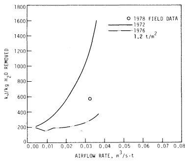
Fig. 9— Electrical energy for fan operation per unit of water removed for a grain-mass/collector-area ratio of 1.2 t/m 2 . Grain depth: 4.6 m (central Iowa).
