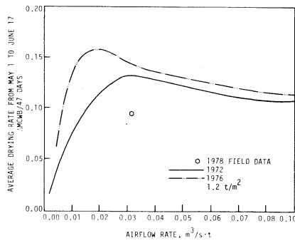
Fig. 3—Average drying rate vs. airflow rate for a grain-mass/collector-area ratio of 1.2 t/m 2 (central Iowa).
