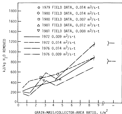
Fig. 12— Electrical energy for fan operation vs. grain mass/collector-area (central Iowa).
