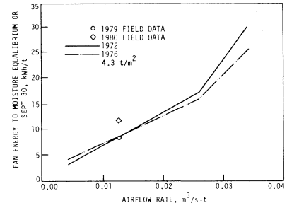
Fig. 8—Electrical energy for fan operation per unit grain mass vs. airflow rate for a grain mass/collector-area ratio of 4.3 t/m 2 (central Iowa).
