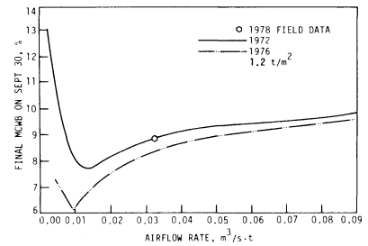
Fig. 5—Final grain moisture content vs. airflow rate for grain-mass/collector-area ratio of 1.2 t/m 2 (central Iowa).
