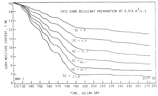
Fig. 1—Corn moisture content vs. time for 1972 solar corn desiccant preparation in central Iowa.
