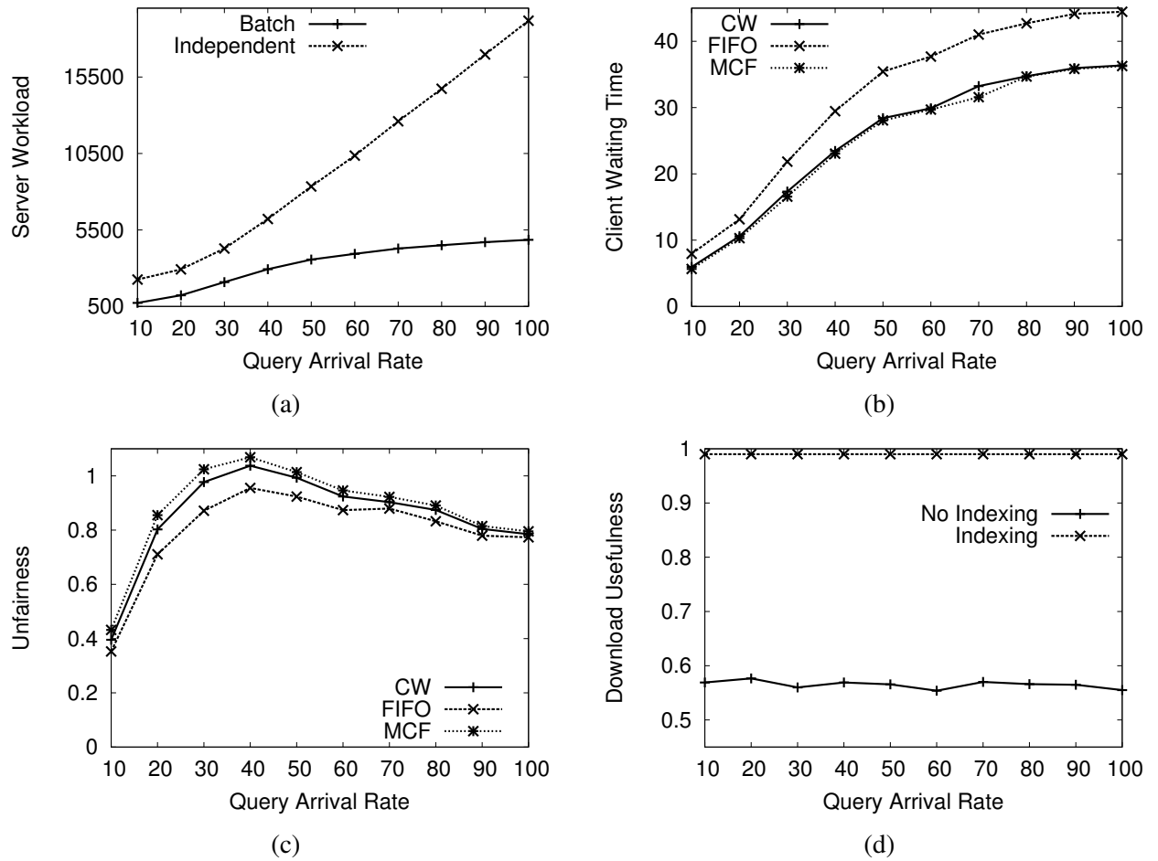
Figure 3.5 Impact of query arrival rate
