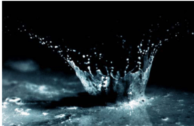
Raindrop splash and displacement of soil particles. Source: USDA Natural Resources Conservation Service.
