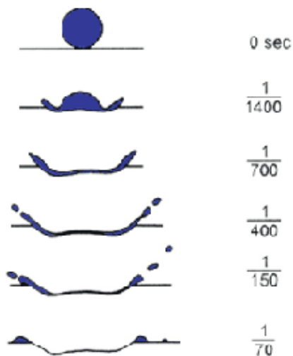
Figure 1. Sequential profile of a raindrop splash pattern. (Source: Environmental Soil Physics, Hillel)
