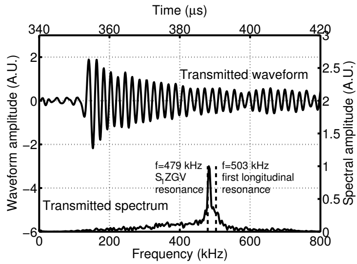
Figure 2: Waveform and spectrum of broadband signal transmitted through glass.
