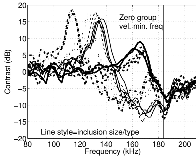
Figure 7: Contrast of inclusions relative to background as a function of scan frequency.
