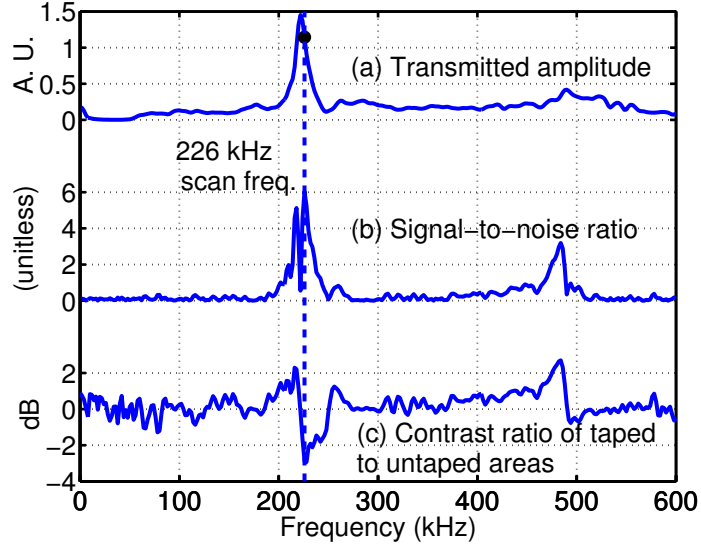
Figure 5: Variation in quality parameters of the image in Fig. 4 as scan frequency is varied: (a) Transmitted amplitude, (b) Signal-to-noise ratio, (c) Contrast ratio of taped to untaped areas of Lucite.
