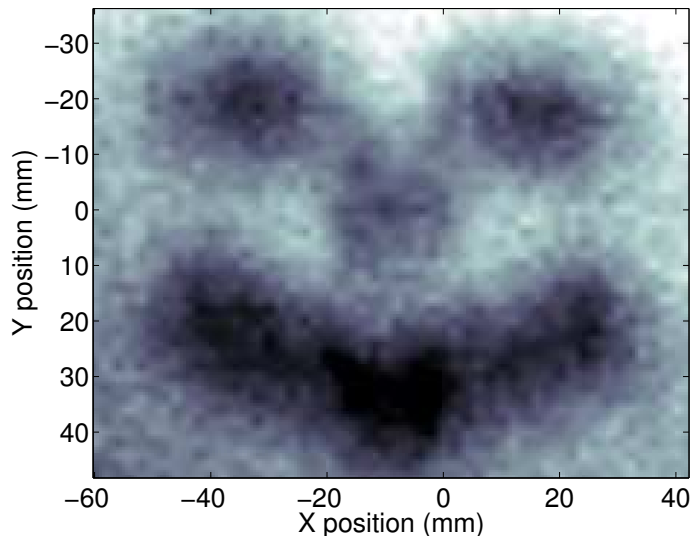
Figure 4: Image of a pattern of scotch tape on Lucite, 226 kHz.
