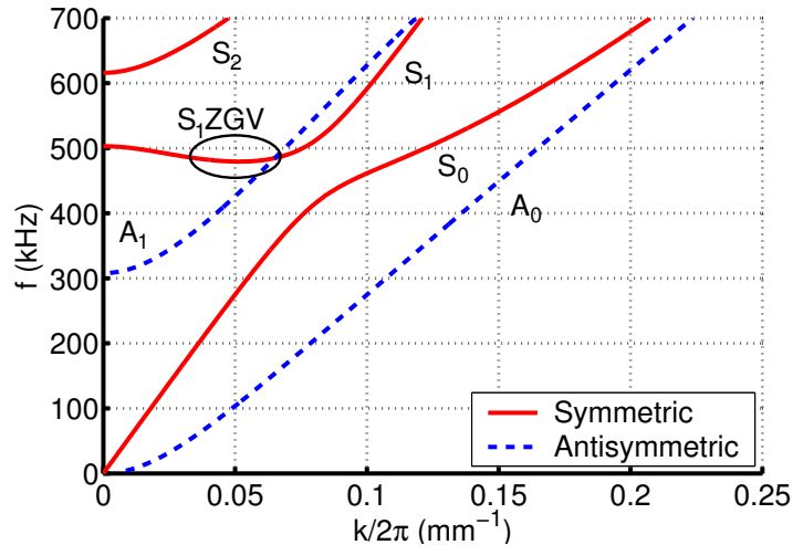
Figure 1: Calculated dispersion relation for 5.72-mm glass. c_l=5.8 mm/ \mu s, c_s=3.5 mm/ \mu s, \rho=2500 kg/m 3 .
