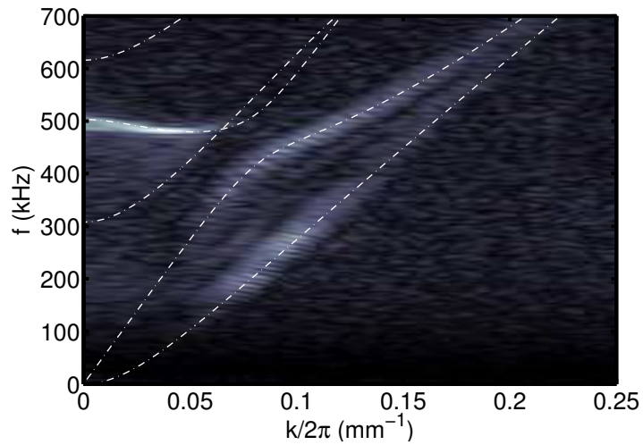
Figure 3: Measured dispersion spectrum for 5.72-mm glass. The calculated curves of Fig. 1 are superimposed as dashed lines.
