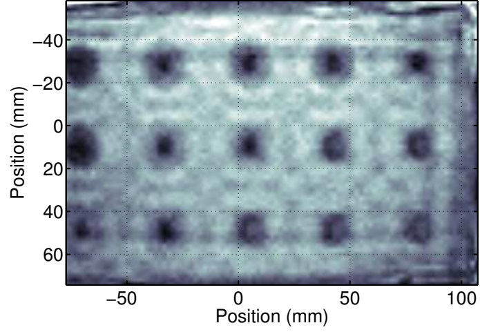
Figure 6: 184 kHz scan of carbon fiber epoxy with 3.2-6.4 mm Teflon inserts
