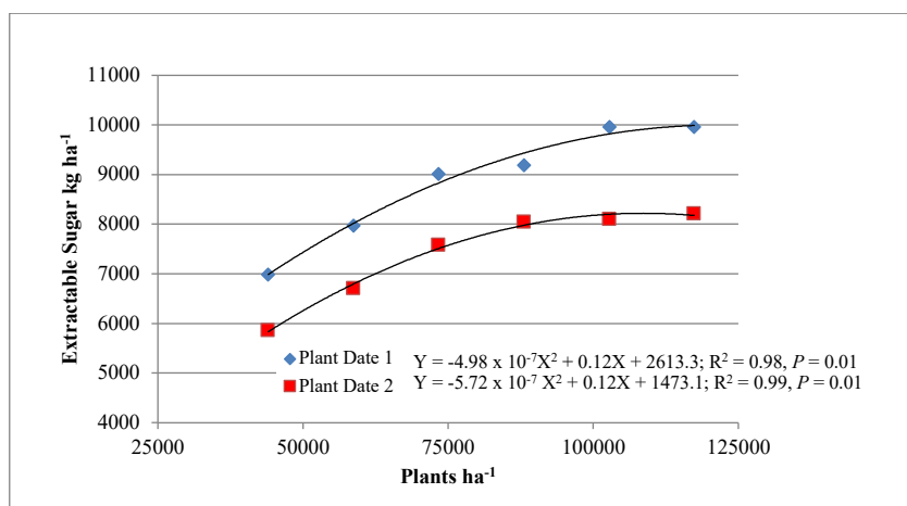
Figure 3. Extractable sugar yield (kg ha -1 ) by plant population for planting date one and planting date two.
