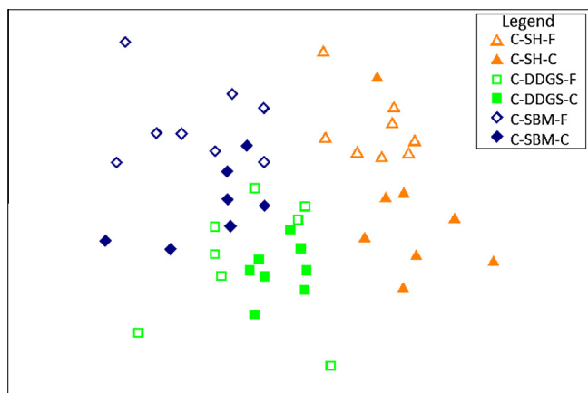
Fig. 6. Non-metric multidimensional scaling plot based on the ARISA analysis (S17 Bray Curtis similarity) to illustrate differences in microbial community as a result of fiber source and grind size. FSBM – fine ground soybean meal, CSH – coarse ground soybean hulls, CDDGS – coarse ground DDGS, FSH – fine ground soybean hulls, FDDGS – fine ground DDGS, and CSBM – coarse ground soybean meal.
