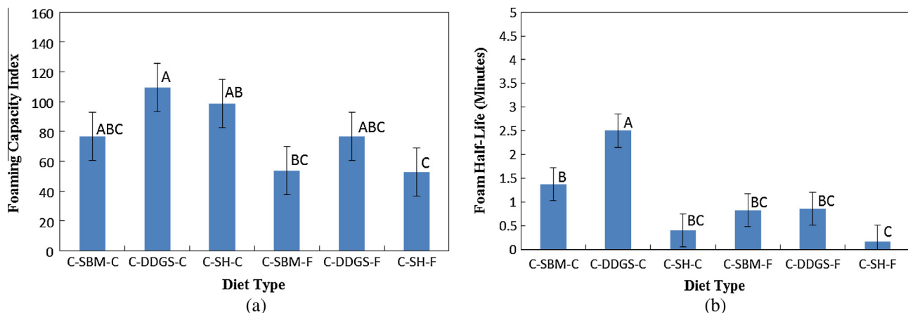
Fig. 5. Average foaming capacity (a) and foam stability (b) for C-SBM-C (Corn-Soybean Meal-Coarse), C-DDGS-C (Corn-DDGS-Coarse), C-SH-C (Corn-Soybean Hulls-Coarse), C-SBM-F (Corn-Soybean Meal-Fine), C-DDGS-F (Corn-DDGS-Fine), C-SH-F (Corn-Soybean Hulls-Fine). Error bars represent the standard error of the mean and capital letters indicate differences ( \alpha = 0.05 ).
