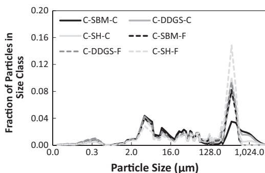
Fig. 2. Particle sizes of the manure from pigs fed the different diets C–SBM–C (Corn–Soybean Meal–Coarse), C–DDGS–C (Corn–DDGS–Coarse), C–SH–C (Corn–Soybean Hulls–Coarse), C–SBM–F (Corn–Soybean Meal–Fine), C–DDGS–F (Corn–DDGS–Fine), C–SH–F (Corn–Soybean Hulls–Fine).
