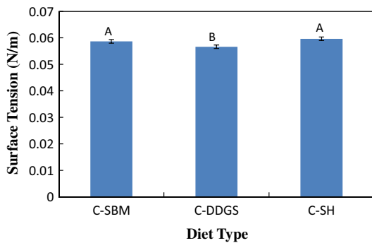
Fig. 4. Average surface tension of the manure samples obtained from different diet fiber sources C-SBM (Corn-Soybean Meal), C-DDGS (Corn-DDGS), C-SH (Corn-Soybean Hulls). Error bars represent the standard error of the mean and capital letters indicate differences ( \alpha = 0.05 ).
