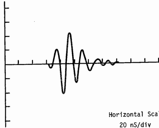
Fig. 3. (A) Insertion loss versus normalized frequency plot of a typical PSN/fused \text{SiO}_2 transducer (50 MHz center frequency); impulse response of a typical PSN/fused \text{SiO}_2 transducer (50 MHz center frequency) (B) experimental impulse response, and (C) theoretical impulse response.
