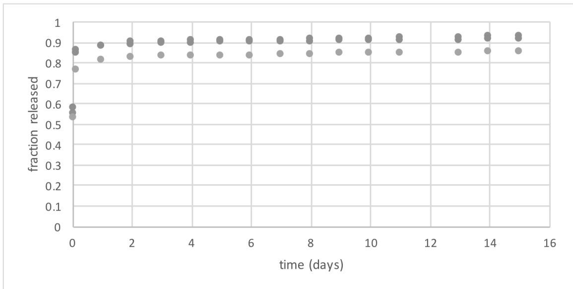
Figure 12. Release kinetics of fludioxonil loaded CPTEG:CPH nanoparticles over 16 days at 37°C. Data were collected by Dr. Balaji Narasimhan (professor) and Adam S. Mullis (graduate research assistant), Department of Chemical and Biological Engineering, Iowa State University of Science and Technology, 2017.
