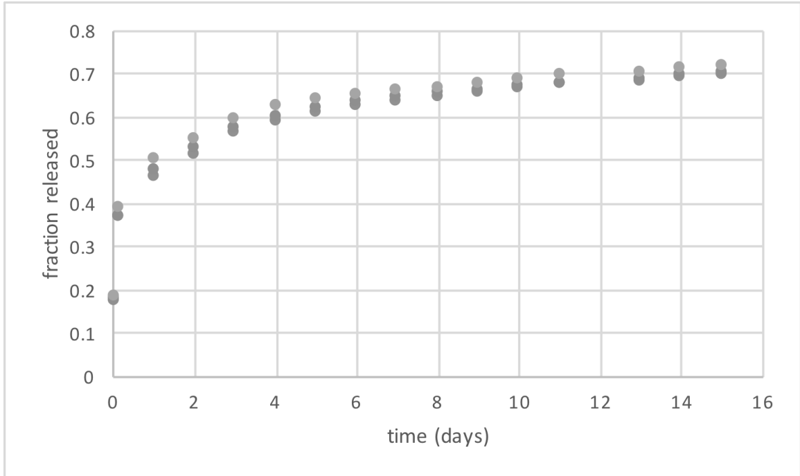
Figure 11. Release kinetics of thiabendazole loaded CPTEG:CPH nanoparticles over 16 days at 37°C. Data were collected by Dr. Balaji Narasimhan (professor) and Adam S. Mullis (graduate research assistant), Department of Chemical and Biological Engineering, Iowa State University of Science and Technology, 2017.
