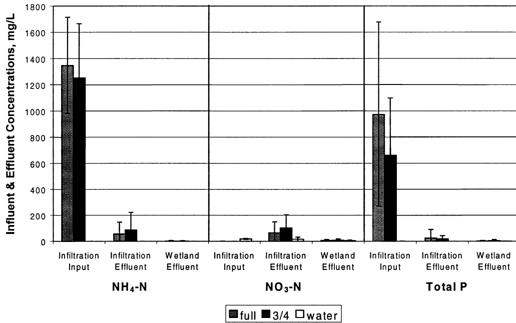
Figure 5. Average nutrient concentrations for the soil infiltration and wetland treatment system for 1999. Bars indicate the standard deviation of each value.
