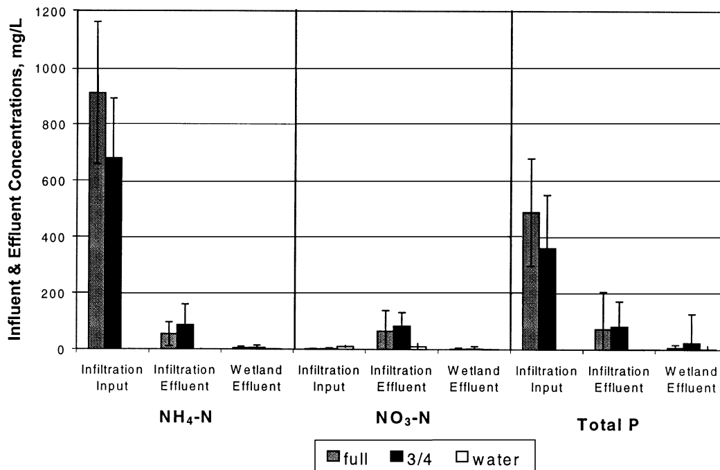
Figure 4. Average nutrient concentrations for the soil infiltration and wetland treatment system for 1998. Bars indicate the standard deviation of each value.
