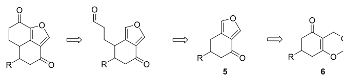
Scheme 1. Retrosynthetic analysis
