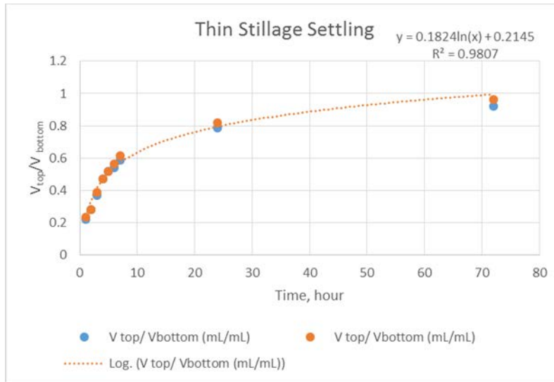
Figure 19. Top volume vs. bottom volume changes in thin stillage
