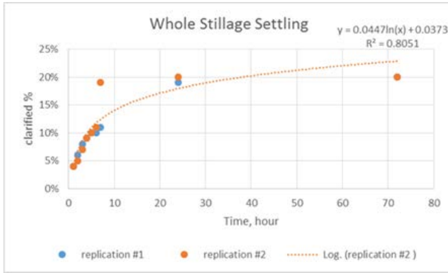
Figure 14. Top volume changes in whole stillage
