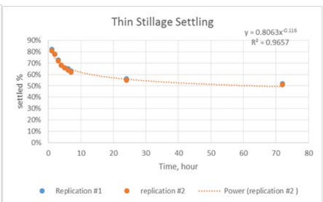
Figure 18. Bottom volume changes in thin stillage
