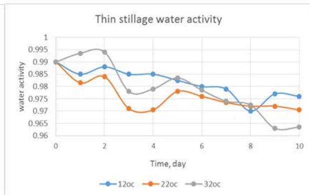
Figure 8. Water activity changes in thin stillage
