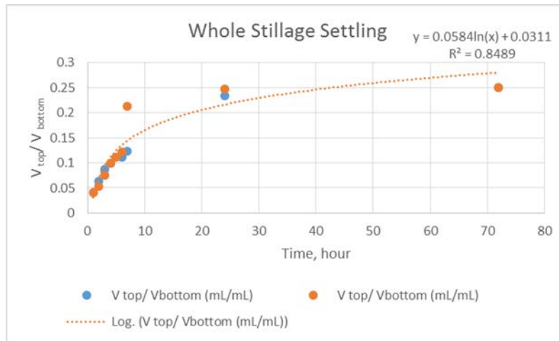
Figure 16. Top volume vs. bottom volume changes in whole stillage
