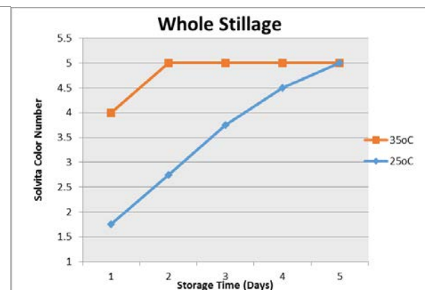
Figure 26. % Solvita® number vs. storage time of whole stillage
