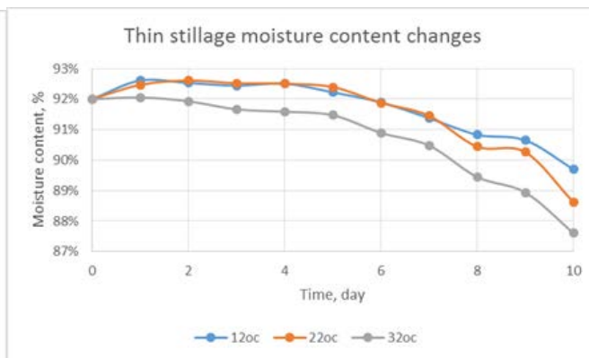
Figure 5. Moisture changes in thin stillage
