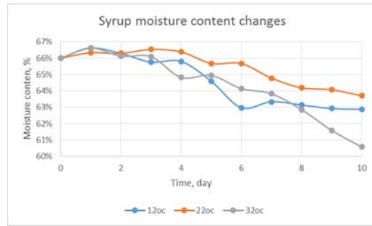
Figure 6. Moisture changes in syrup
