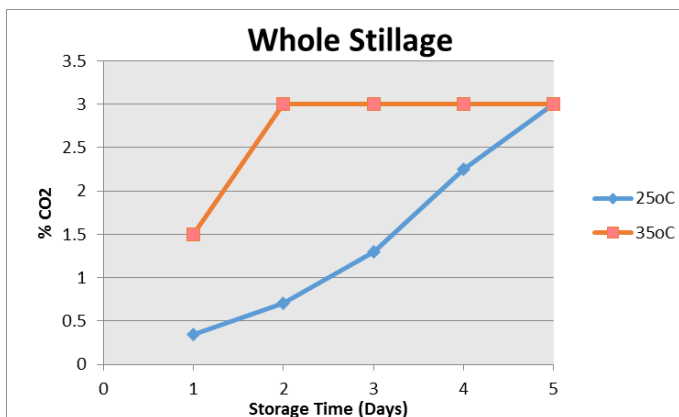
Figure 25. % CO 2 vs. storage time of whole stillage
