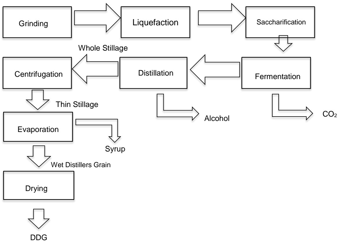
Figure1. Ethanol production process overview.
