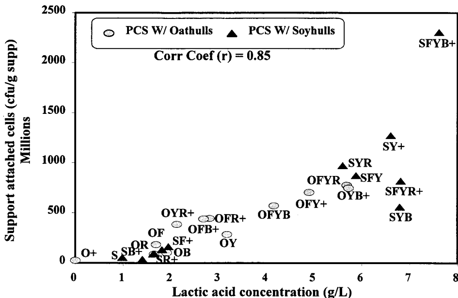
FIG. 5. Relationship between L. casei biofilm population on supports (supp) and lactic acid production during BF. The least significant difference ( P < 0.05 ) of viable cells attached on supports and lactic acid concentration were 5.7 \times 10^8 CFU/g of support and 2 g/liter, respectively. See Table 1 for support compositions.
