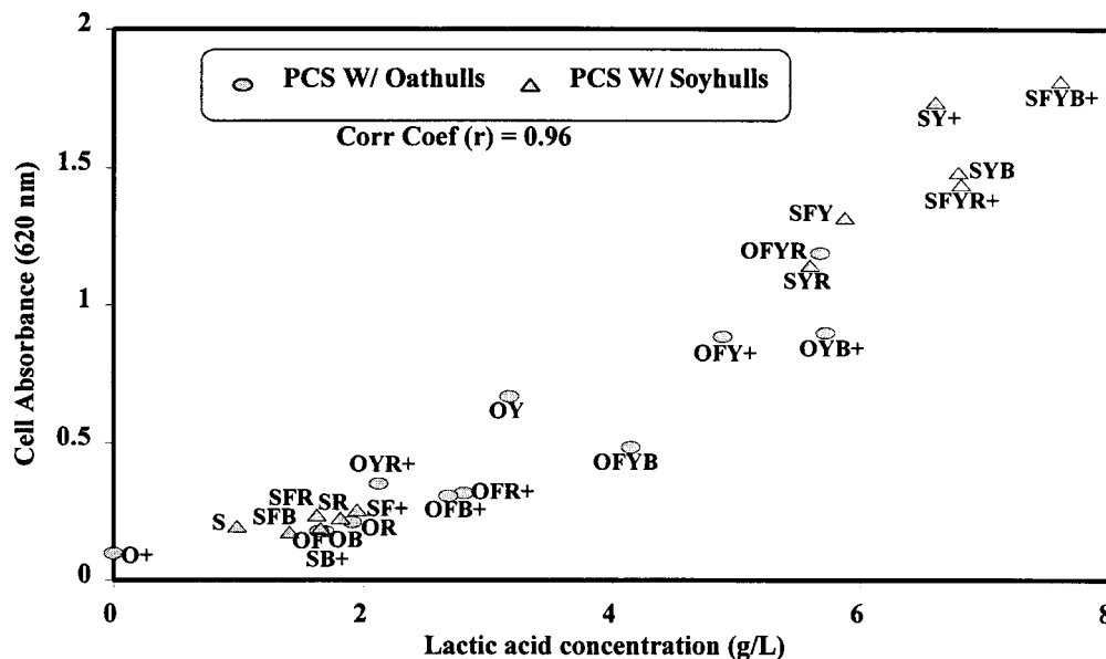
FIG. 4. Relationship between L. casei suspended-cell density in MM and lactic acid production during BF. The least significant difference ( P < 0.05 ) of cell density and lactic acid concentration were absorbance of 0.58 and 2 g/liter, respectively. See Table 1 for support compositions.
