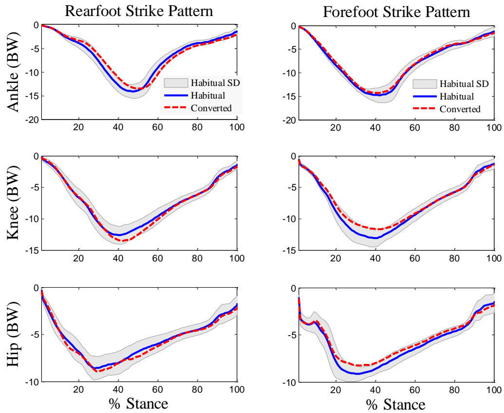
Figure 3: Comparison of axial contact forces at ankle, knee, and hip between habitual and converted strike patterns. Negative values represent compression. Note the difference in scaling between joints.
