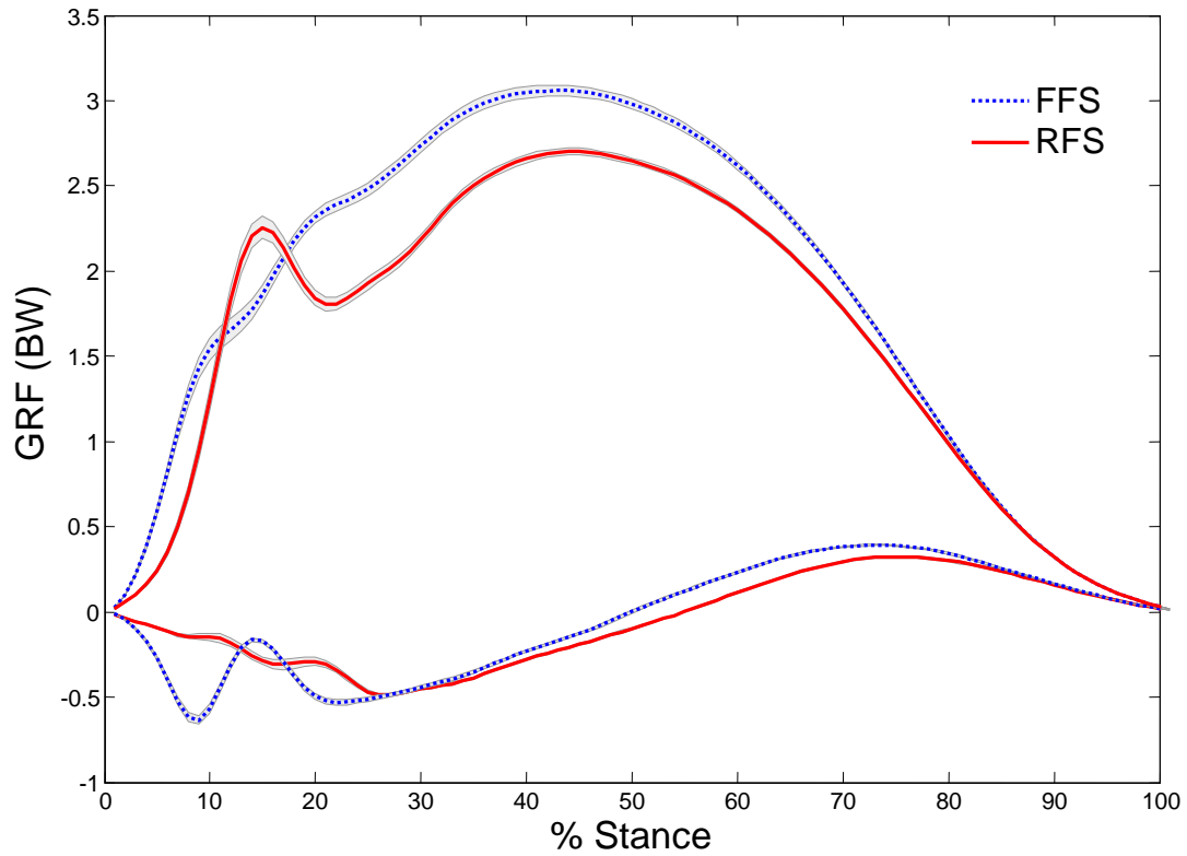
Figure 5: Ensemble curves for vertical and AP GRF during FFS and RFS running. The solid line represents RFS and the dotted represents FFS. Positive values represent forces in the vertical and anterior direction. (note: I need to add a legend on the graph and change it so that it is obvious what is RFS and FFS)
