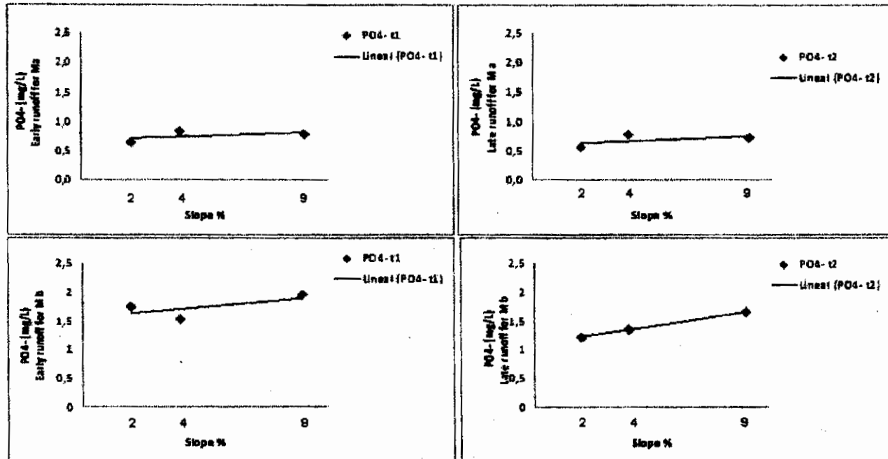
Fig. 4. PO 4 (mg/L) at early and late runoff (t1 and t2), for Ma and Mb manure concentrations and different slopes
