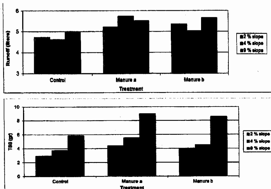
Fig. 2. Runoff and sediment yield at different slopes. a) Mean runoff volume per treatment (in Liters); b) Mean sediment yield (TSS) per treatment (in grams)
