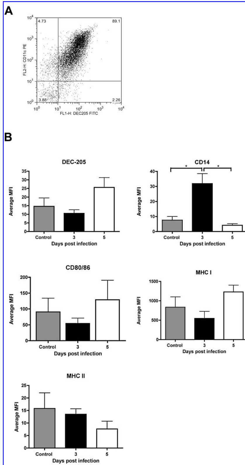
FIG. 3. BRSV infection of neonatal ovine lungs induces modulation of surface antigen expression on CD11c + lung DCs. Lung DCs were sorted magnetically to purify CD11c + cells from digested neonatal lung suspensions from controls, day 3 postinoculation lambs, and day 5 postinoculation lambs. Flow cytometric analysis of surface antigen expression revealed that 89% of the sorted lung DCs coexpressed CD11c and DEC-205 (A). Statistical analysis indicated a higher mean fluorescence intensity (MFI) expression of CD14 on lung DCs isolated on day 3 postinoculation when compared with controls or day 5 postinoculation lung DCs (B) (* p < 0.05). MHC class I and CD80/86 expression was higher on isolated lung DCs from day 5 postinoculation lambs. Each column represents the average of the MFI staining for the indicated cell surface antigen minus the MFI staining of the appropriate isotype control. Data are representative of two experiments with six lambs per experimental group.
