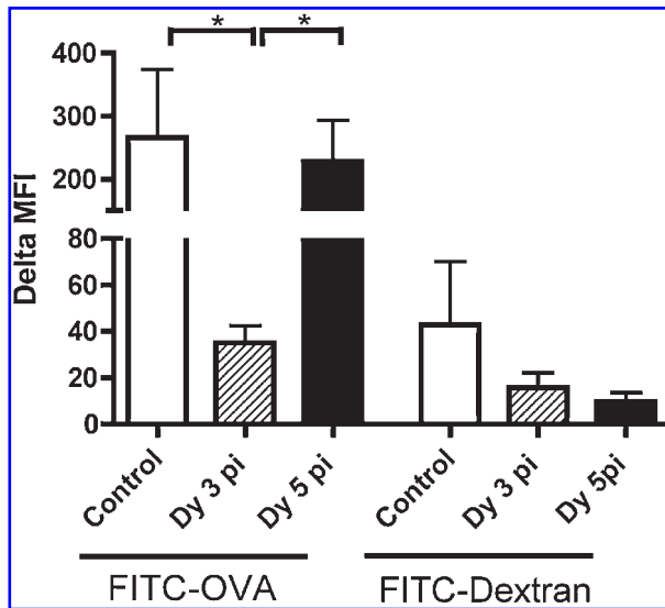
FIG. 4. Uptake of FITC-ovalbumin (FITC-OVA) and FITC-dextran by isolated lung DCs. Magnetically sorted CD11c + lung DC cell numbers were adjusted to 1 \times 10^5 cells/mL and incubated with either FITC-OVA or FITC-dextran for 1 h at 37 or 4°C. Data are expressed as the change in mean fluorescence intensity (MFI) values, that is, the 37°C MFI values minus the 4°C MFI values. Statistical analyses indicate that lung DCs on day 3 postinoculation endocytosed less FITC-OVA than either the controls or day 5 postinoculation lung DCs ( *p < 0.05 ). Data are representative of two experiments with six lambs per treatment group.
