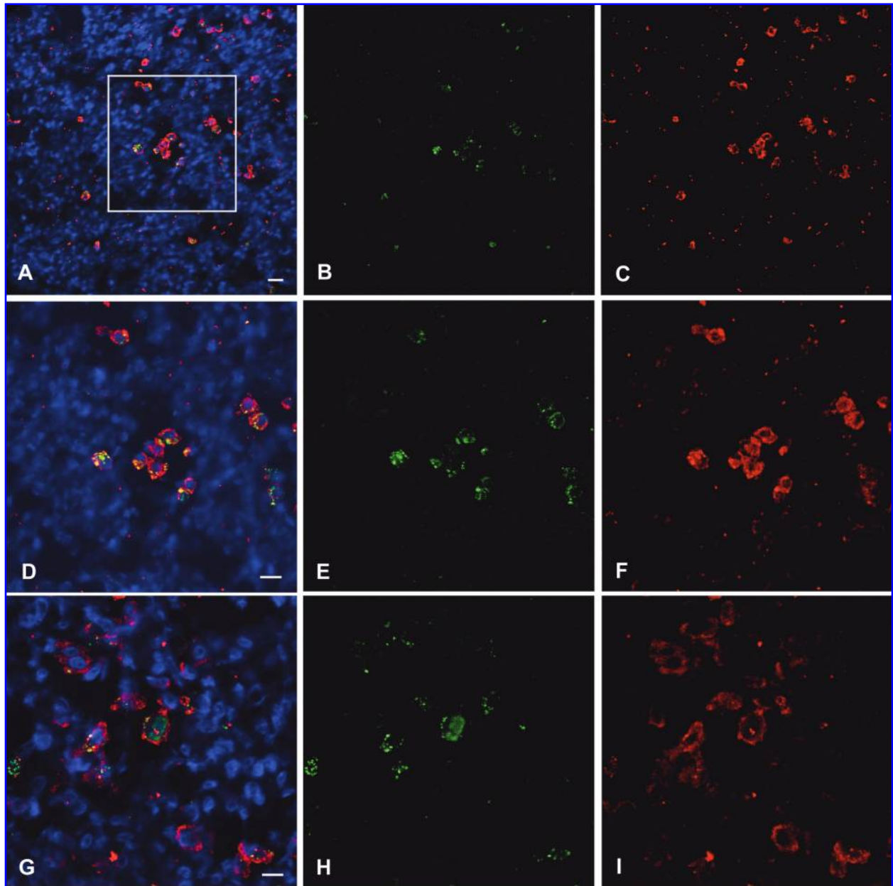
FIG. 1. BRSV antigen colocalizes with CD11c + cells in the lungs of neonatal lambs. Neonatal ovine lung cryosections were immunofluorescently stained with a primary antibody directed against CD11c ( C , F , and I ) followed by a secondary antibody fluorescently labeled with Alexa Fluor 633 (red). Directly conjugated BRSV-FITC ( B , E , and H ) antibody (green) was used to identify cells containing BRSV. Coexpression of CD11c and the virus is shown by yellow. Multicolor immunofluorescence staining shows dual-labeled DCs ( A , D , and G ) and nuclear staining with DAPI (blue). The enlarged view ( D–F ) is of the inset in ( A ) and an additional and different enlarged view ( G–I ) reveals more CD11c and BRSV colocalization. Data are representative of two experiments with 12 infected lambs. Scale bars: ( A–C ) 20 \mu m; ( D–I ) 10 \mu m.
