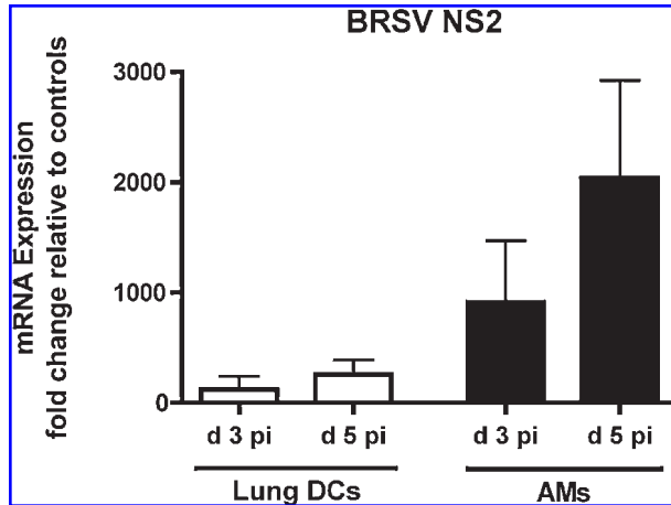
FIG. 2. BRSV replicates within lung dendritic cells (DCs) and alveolar macrophages (AMs). Isolated lung DCs and AMs were lysed in RLT buffer and total RNA was isolated. Oligo(dT) cDNA and BRSV NS2-specific primers with SYBR green chemistry were used for quantification of viral replication. Lung DCs supported BRSV replication, but less so than AMs. Data are representative of two experiments with six lambs per treatment group. Pi, Postinoculation.
