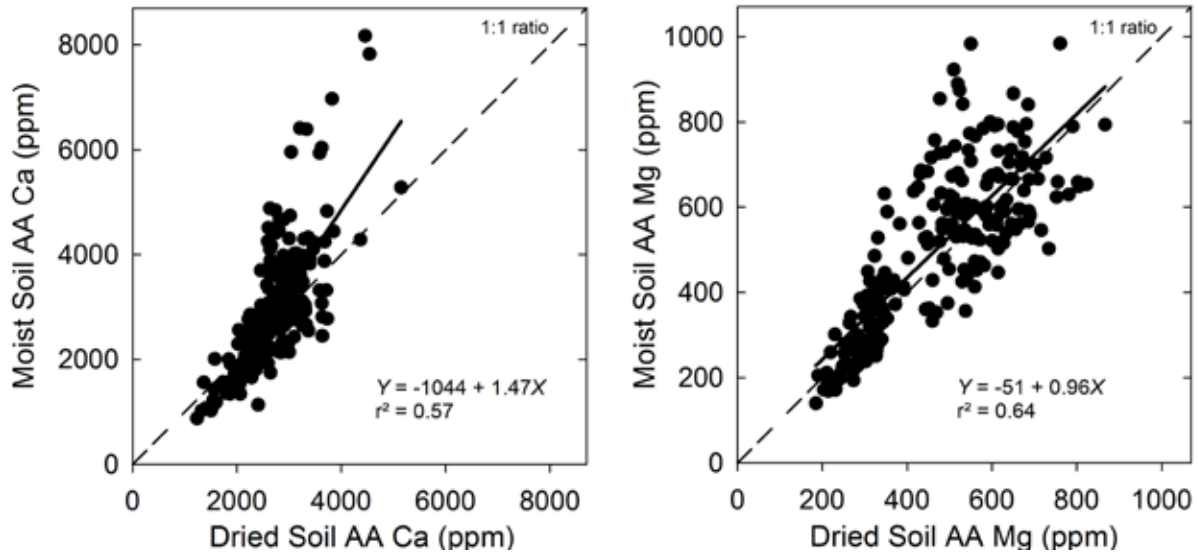
Figure 5. Relationship between Ca and Mg measured on moist or dried samples using the ammonium-acetate (AA) method.
