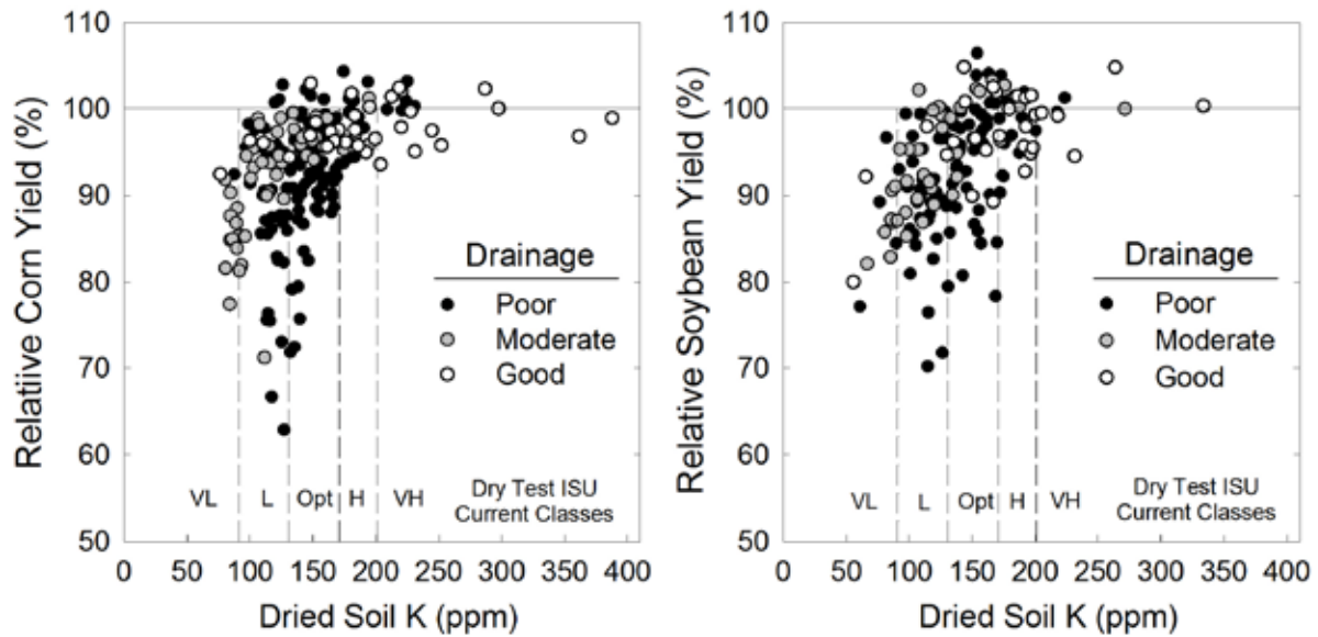
Figure 7. Relationship between relative corn and soybean yield response to K and soil-test K measured on dried samples. Symbols identify data for soil series with different drainage. VL, L, Opt, H, and VH identify current ISU very low, low, optimum, high, and very high interpretation classes for the dry test.
