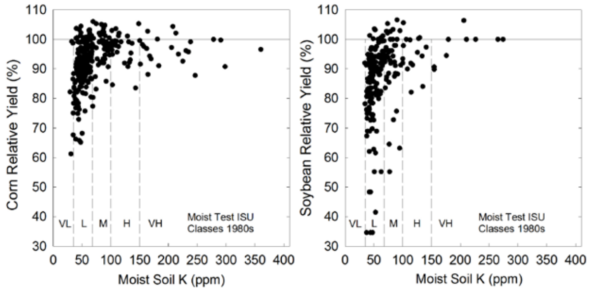
Figure 1. Relationship between relative corn and soybean yield response to K and soil-test K measured on moist samples for data collected from 1976 until 1989 (Mallarino et al., 1991). VL, L, M, H, and VH identify the 1982 ISU very low, low, medium, high, and very high interpretation classes for the moist test.
