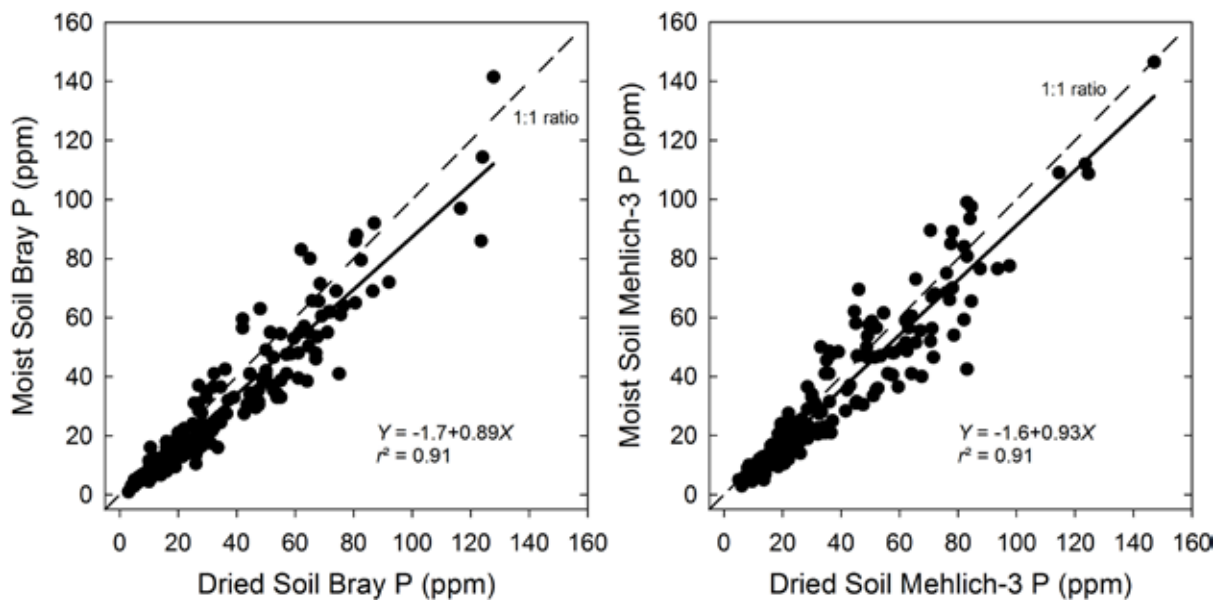
Figure 4. Relationship between P measured on moist or dried samples using the Bray-1 and Mehlich-3 methods (extracted P was measured colorimetrically for both methods).
