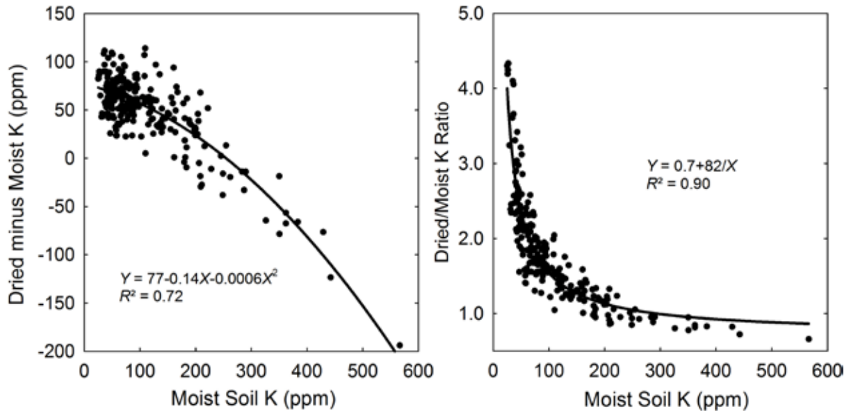
Figure 3. Relationship between the difference or the ratio of K extracted from dried or field-moist soil samples collected and analyzed in 2011.
