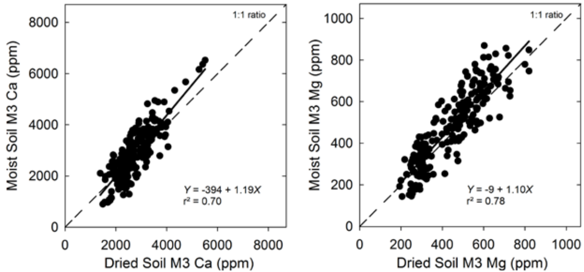
Figure 6. Relationship between soil Ca and Mg measured on moist or dried samples using the Mehlich-3 (M3) method.
