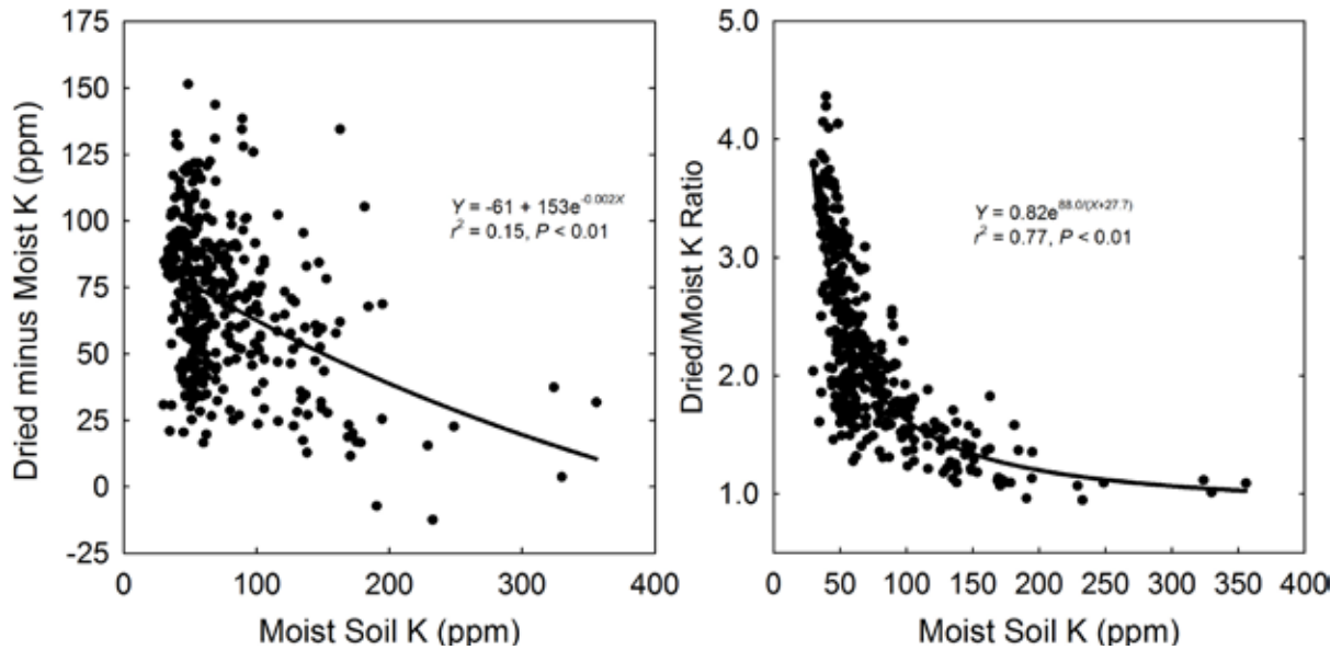
Figure 2. Relationship between the difference or the ratio of K extracted from dried or field-moist soil samples collected and analyzed from 2001 through 2006.
