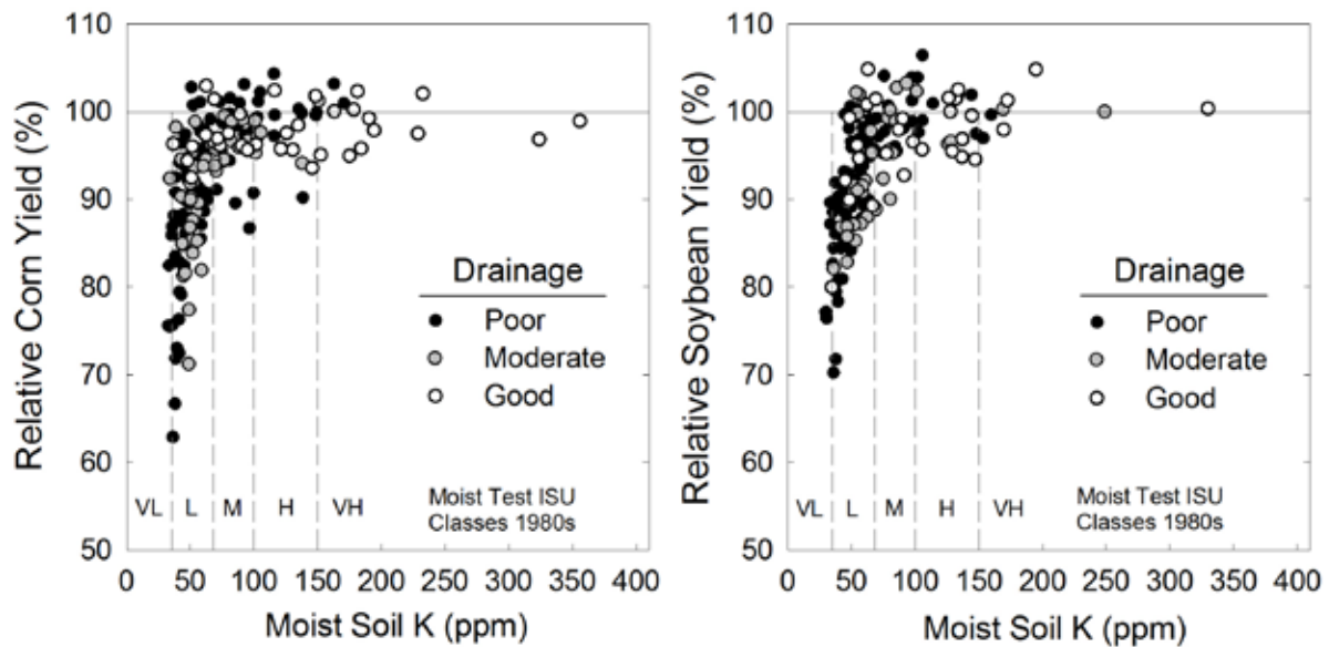
Figure 8. Relationship between relative corn and soybean yield response to K and soil-test K measured on moist samples. Symbols identify data for soil series with different drainage. VL, L, M, H, and VH identify the 1982 ISU very low, low, medium, high, and very high interpretation classes for the moist test.
