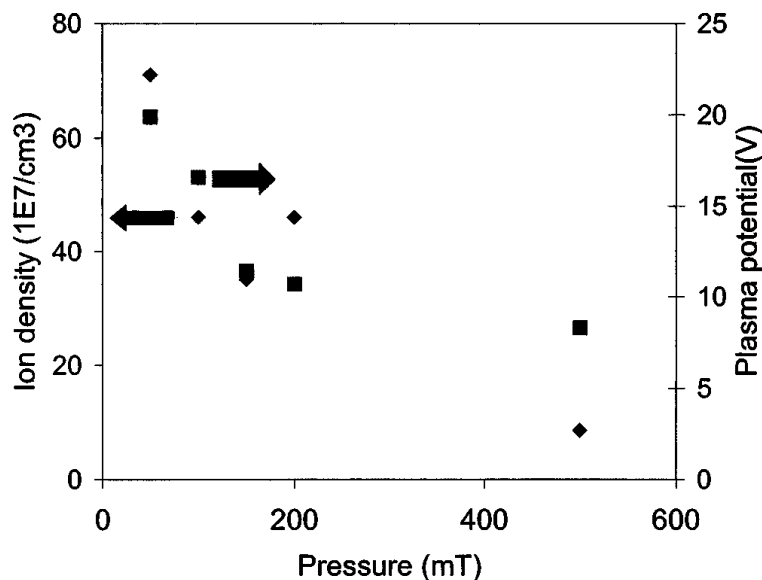
Figure 1.3 Langmuir probe data showing ion density plotted versus chamber pressure. Indicates that both ion density and energy increase with decreasing pressure [12].
