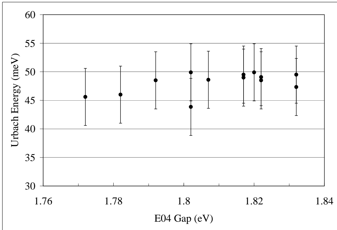
Figure 4.12 Device Urbach energy versus E04 gap.
