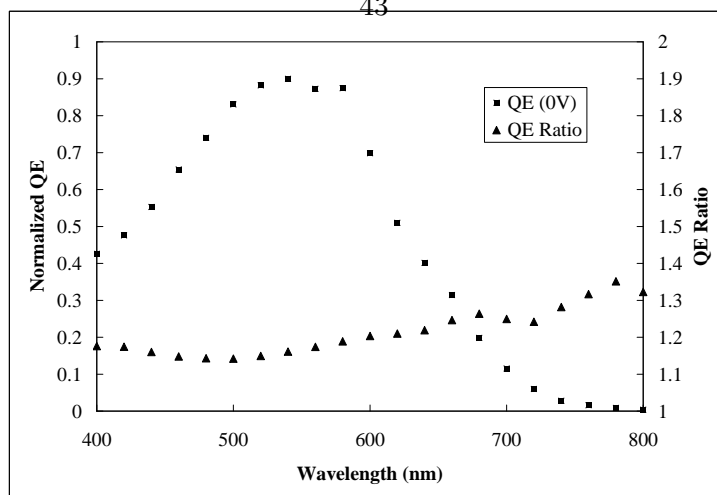
Figure 4.10 Normalized QE and QE ratio versus wavelength plotted. Device fabricated with graded doping in i1 near i1-i2 interface. Device possesses an optical gap of 1.63eV
