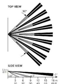
Figure 2. Coverage pattern of the passive IR detection (PID) motion sensor.
